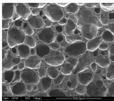
Compound, fine grinding: Q221 micrograph.
