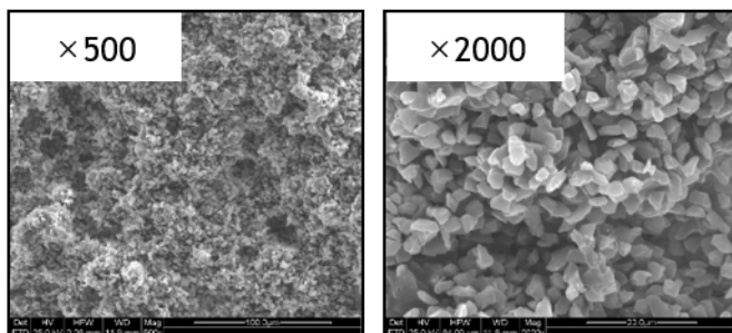
Structure of the #3000-VSPS10 design with both SEM images at \times 500 and \times 2000 ; both original scales retained.
