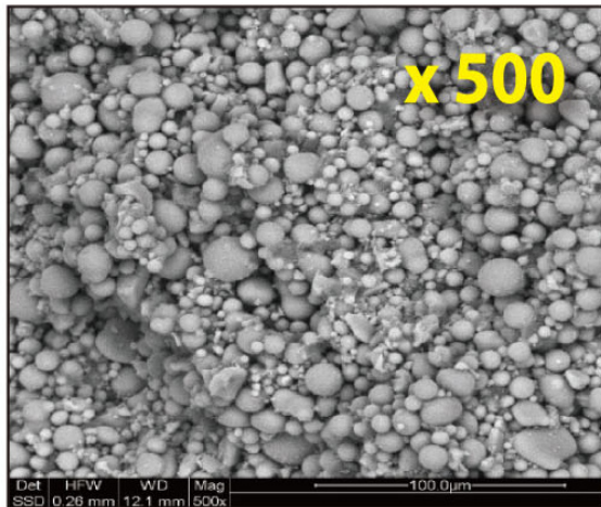
Gettering polishing pad: microstructure X500.
