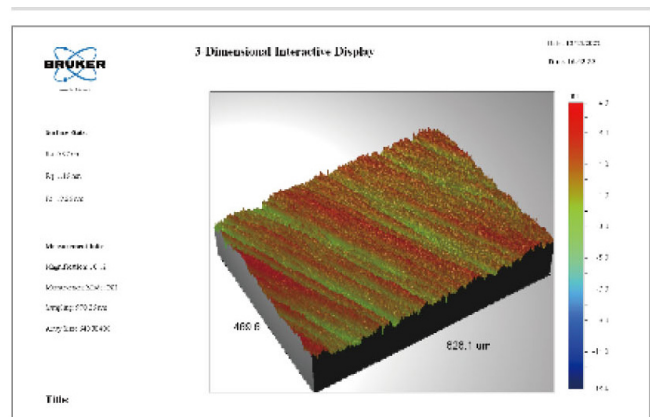
Centre surface: Ra 0.92 nm.
