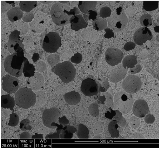
Structure of Z2 design NP-D4-303D3.5W10X-5000-VKBT25; original scale and acquisition labels retained.
