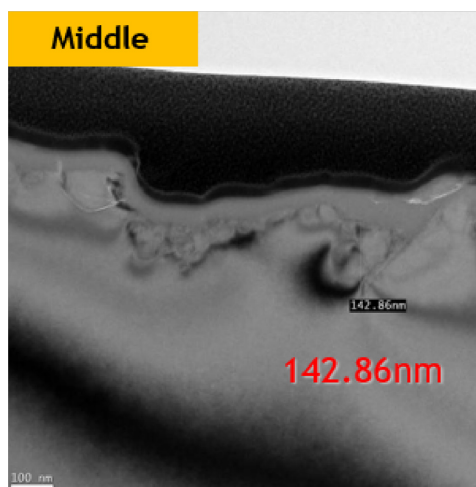
Vitrified #5000, middle: marked damage depth 142.86 nm; original measurement line and scale retained.
