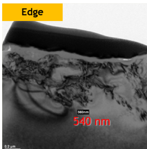
Resin #325, edge: marked damage depth 540 nm; original measurement line and scale retained.
