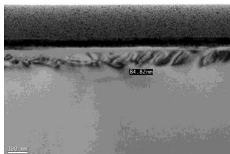
Vitrified #8000, edge: original Q221 measurement image with markings and scale.
