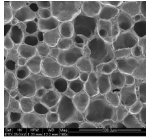
Structure of the #4000-VK8HS design, SEM \times 100 ; original scale retained.
