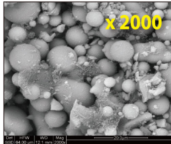
Gettering polishing pad: microstructure X2000.
