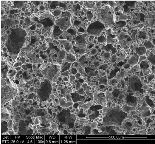
Structure of the #800-VSP3 design, SEM \times 100 ; original scale retained.
