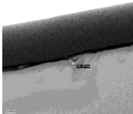
Vitrified #8000, centre: original Q221 measurement image with markings and scale.
