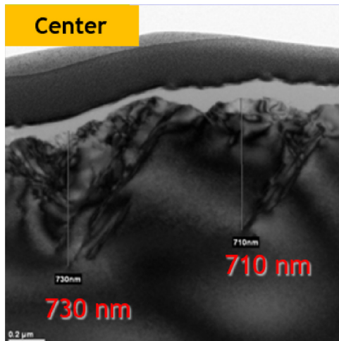
Resin #325, centre: marked damage depths 730 nm and 710 nm; original measurement lines and scale retained.
