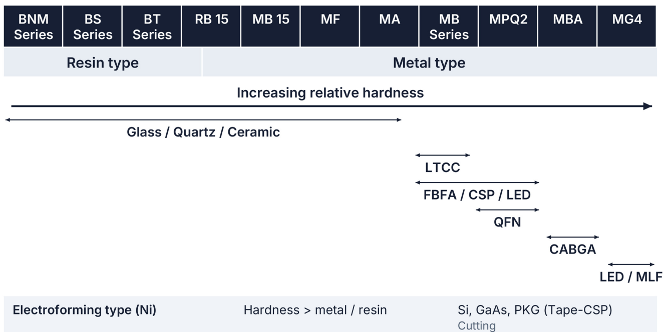
Microblade selection matrix with all series and application ranges.
