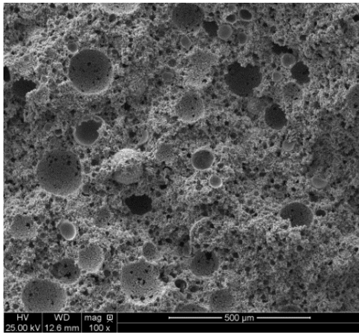
SiC version #2000-VNP8-GC, micrograph with original scale.
