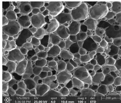
Microstructure of #8000M-VNP-HBF; original scale retained.
