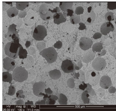
Z2 #5000: combined-sheet micrograph.
