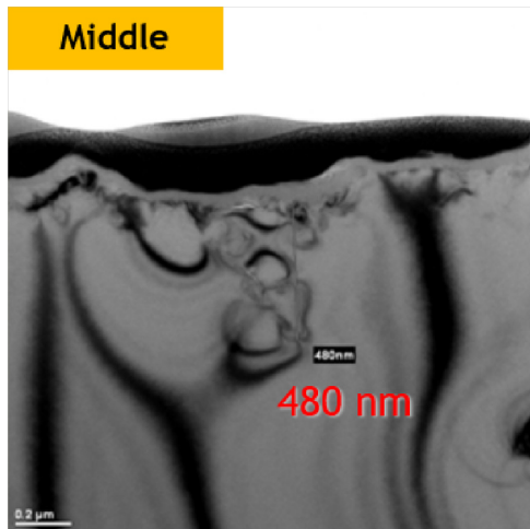
Vitrified #600, middle: marked damage depth 480 nm; original measurement line and scale retained.
