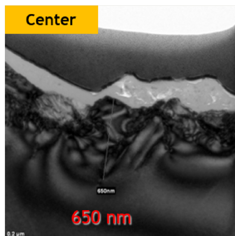
Vitrified #600, centre: marked damage depth 650 nm; original measurement line and scale retained.
