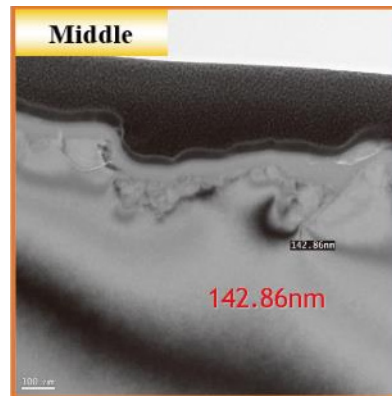
Vitrified #5000, middle: original Q233 measurement image with markings and scale.
