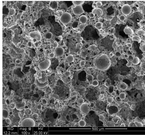
Structure of Z1 design NP-D4-303D3.0W10X-800-VSZT, SEM ×100; original scale retained.
