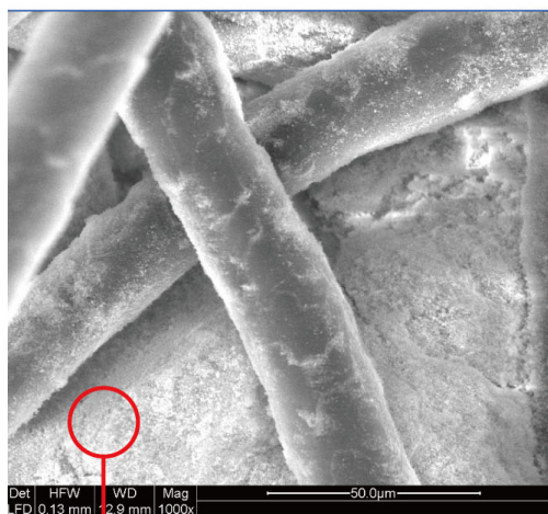
After impregnation: resin and \text{ZrO}_2 .
