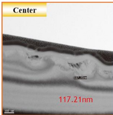
Vitrified #5000, centre: original Q233 measurement image with markings and scale.
