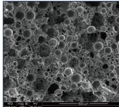
Z1 #600: combined-sheet micrograph.
