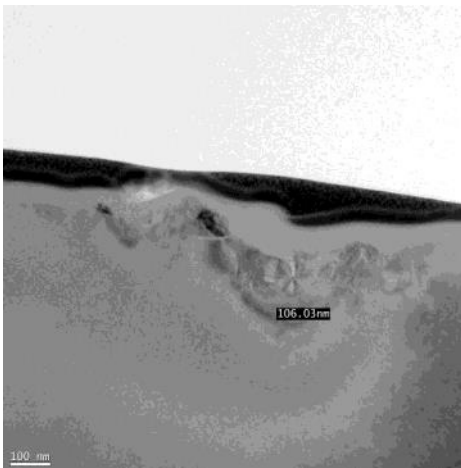
Vitrified #5000, edge: original Q221 measurement image with markings and scale.
