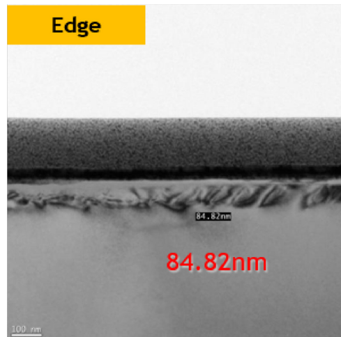
Vitrified #8000, edge: marked damage depth 84.82 nm; original measurement line and scale retained.
