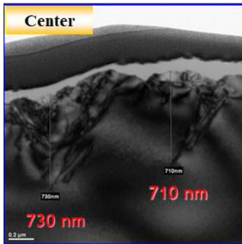
Resin #325, centre: 730 nm and 710 nm.
