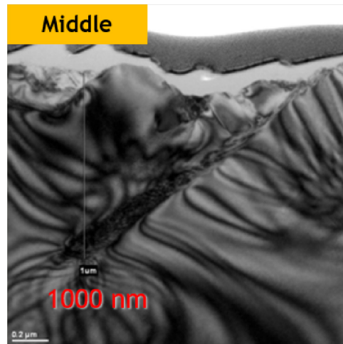
Resin #325, middle: marked damage depth 1000 nm; original measurement line and scale retained.
