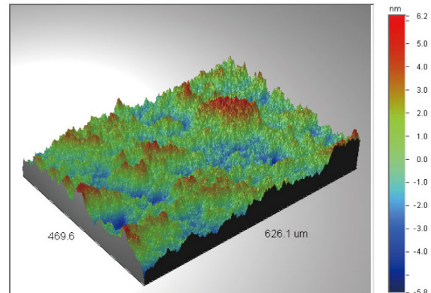
Wyko NT3300: optical 3D surface measurement.
