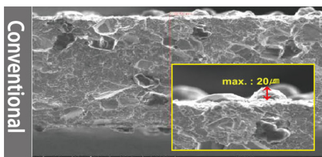
Conventional side surface, original image.
