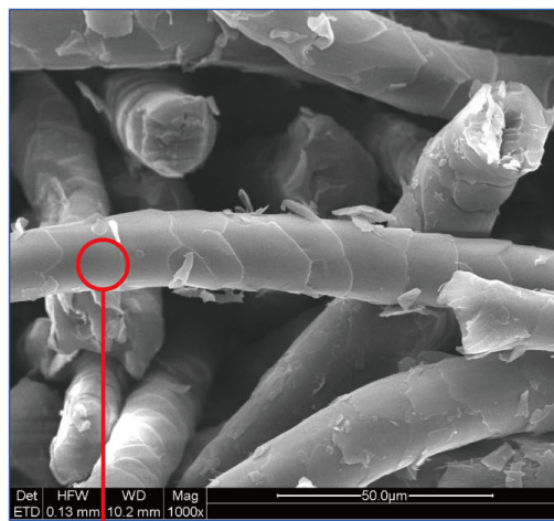
Before impregnation: wool felt.
