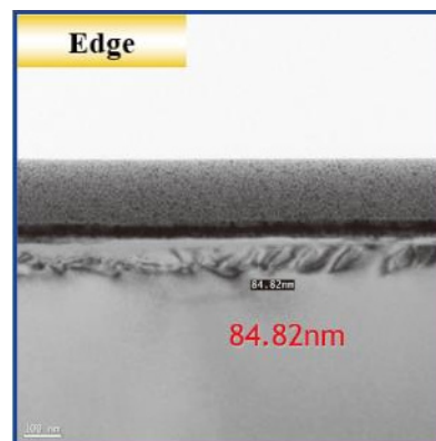
Vitrified #8000, edge: original Q233 measurement image with markings and scale.
