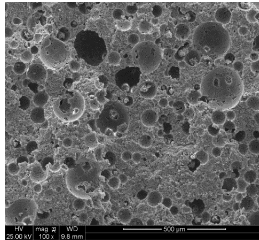
SiC version #8000M2-VNP-PSR, micrograph with original scale.
