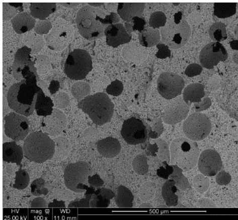
Microstructure of #5000-VKBT25M3-P12; original scale retained.
