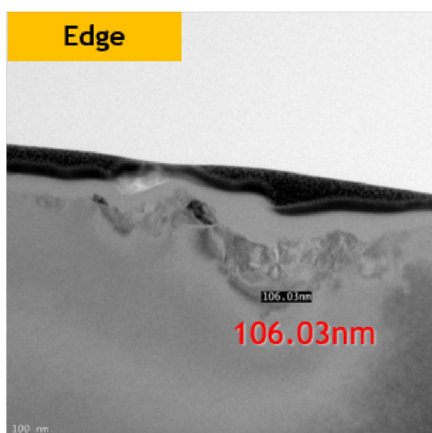
Vitrified #5000, edge: marked damage depth 106.03 nm; original measurement line and scale retained.
