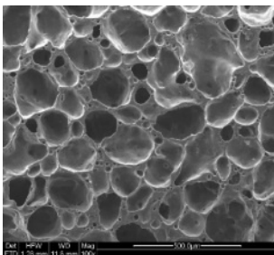
Structure of the #5000-VK8HS design, SEM \times 100 ; original scale retained.
