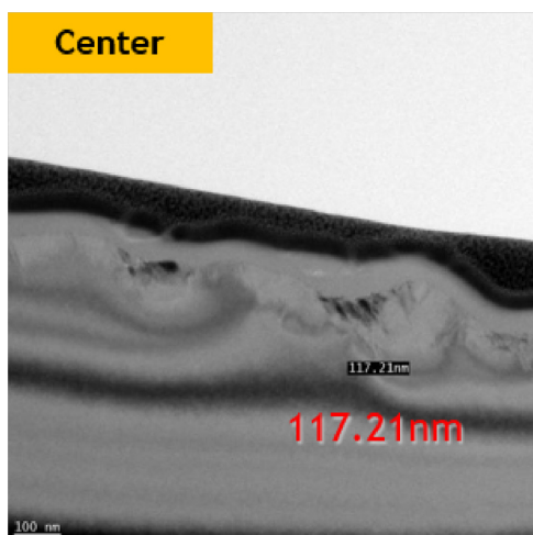
Vitrified #5000, centre: marked damage depth 117.21 nm; original measurement line and scale retained.
