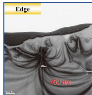
Q233, lower image row, edge: original measurement values and scale retained.
