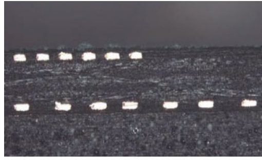
Actual cut image for the side-enhanced version.
