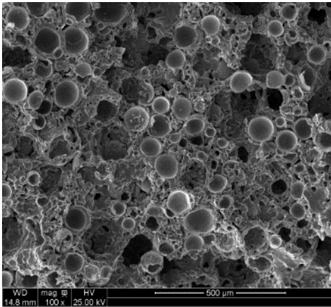
Structure of Z1 design NP-D4-303D3.5W10X-600-VSZT, SEM ×100; original scale retained.
