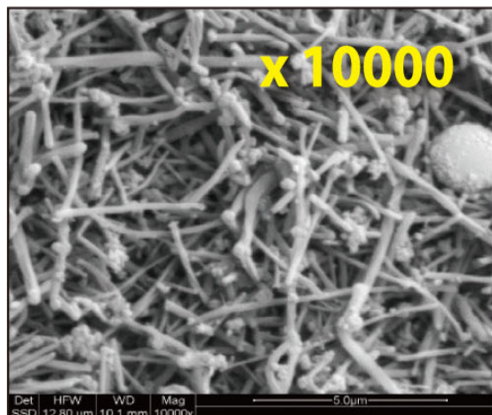
Gettering polishing pad: microstructure X10000.
