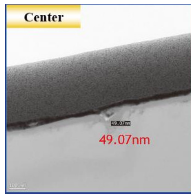
Vitrified #8000, centre: original Q233 measurement image with markings and scale.
