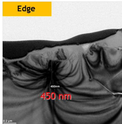
Vitrified #600, edge: marked damage depth 450 nm; original measurement line and scale retained.
