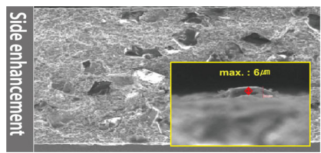
Enhanced side surface, original image.
