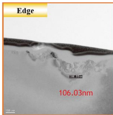
Vitrified #5000, edge: original Q233 measurement image with markings and scale.
