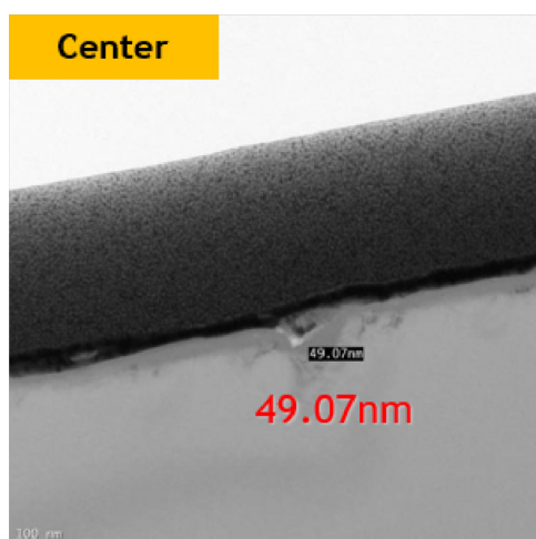
Vitrified #8000, centre: marked damage depth 49.07 nm; original measurement line and scale retained.
