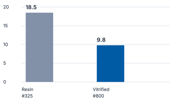
Vertical edge chipping [ \mu\text{m} ]
