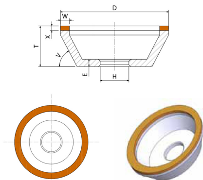
11A2: section, dimension codes and tool model
