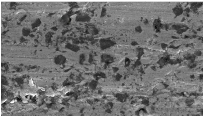
Hybrid-bond microstructure
