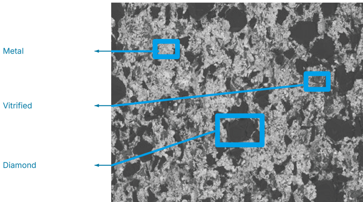
MNC microstructure: metal, vitrified phase and diamond
