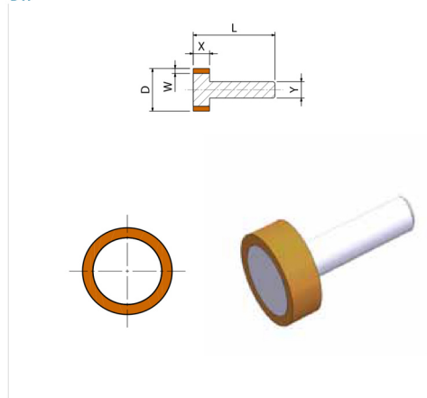
DW: section, dimension codes and tool model
