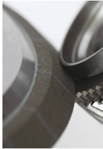
Profiled grinding tools and layer structure
