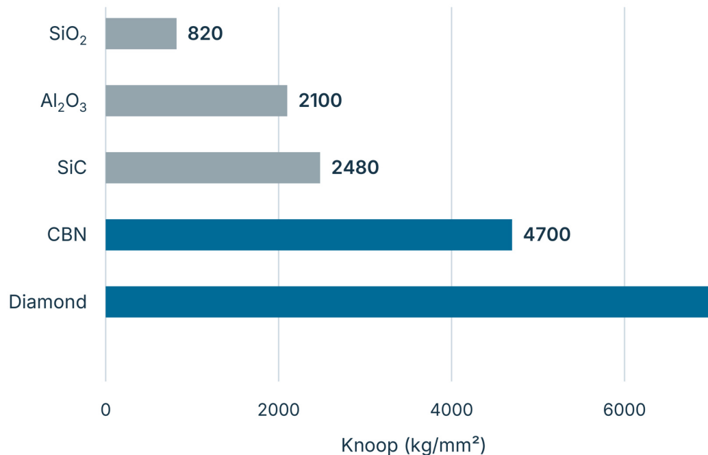
Abrasive hardness comparison: Knoop scale
