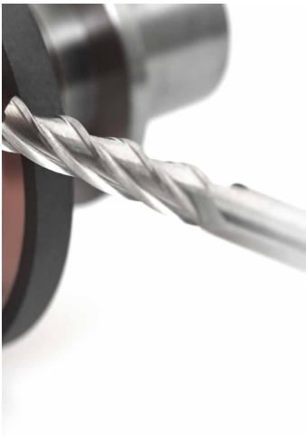
Superabrasive wheel in tool machining
