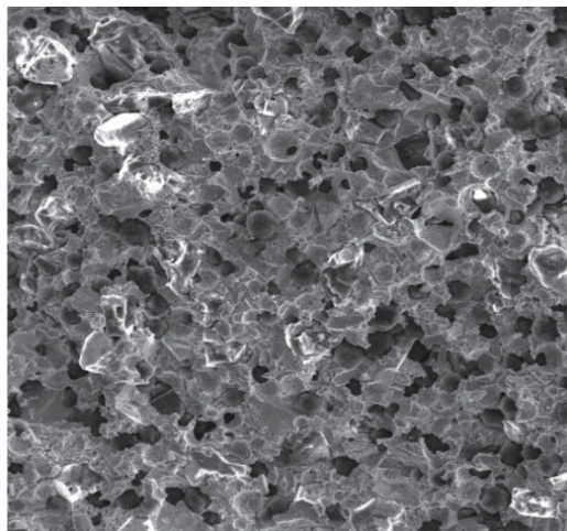
Porous hybrid bond: microstructure 1
