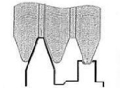
Single and root type: profile contact.
