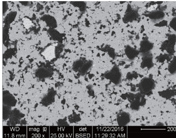
Hybrid-bond microstructure
