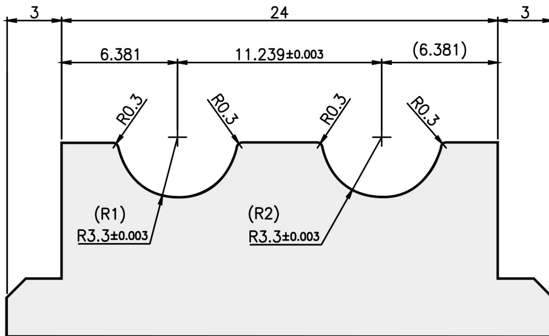
Guide-block profile: dimensions and tolerances
