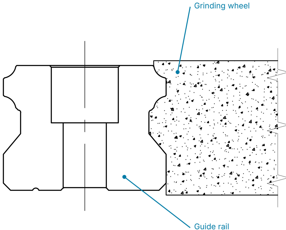
Grinding wheel and guide rail in profile contact
