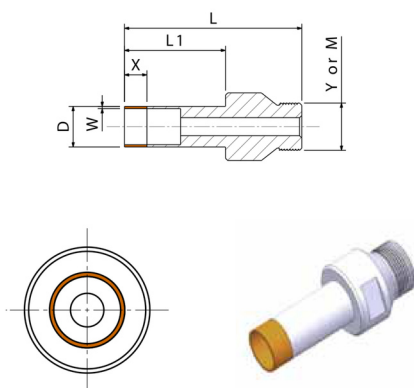
6F2: section, dimension codes and tool model
