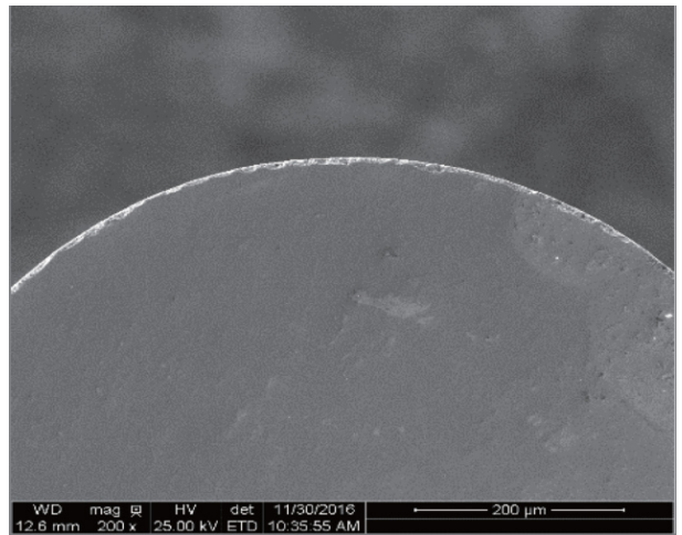
Edge micrograph in the hybrid-bond application example
