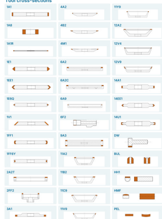
Tool cross-sections
