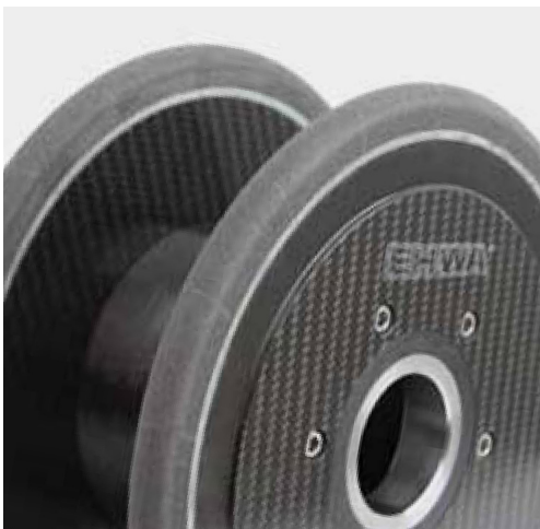
Vitrified grinding wheels with CFRP bodies
