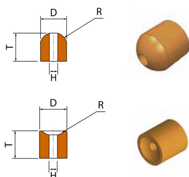
BUL: section, dimension codes and tool model
