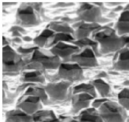
Surface structure of a lens grinding wheel
