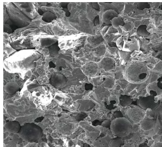
Porous hybrid bond: microstructure 2
