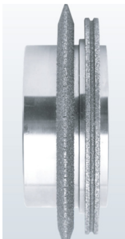
Single & Root: tool view
