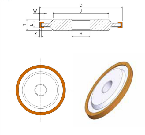
14U1: section, dimension codes and tool model
