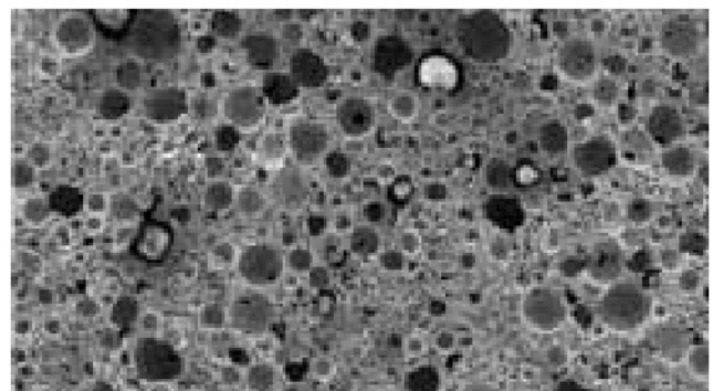
CBN honing stone: coarse pore structure
