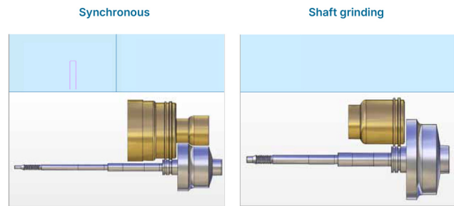
Turbocharger machining arrangements: synchronous and shaft grinding.
