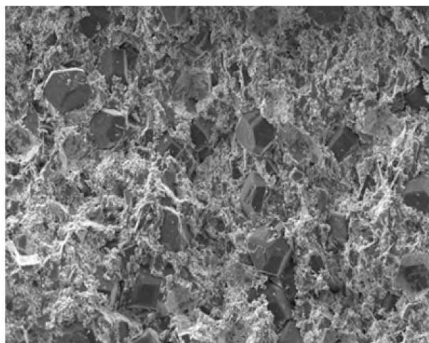
MNC-bond microstructure
