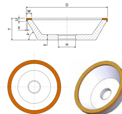
11C9: section, dimension codes and tool model
