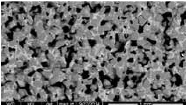
Pore structure of the vitrified-bonded wheel for the outer race.
