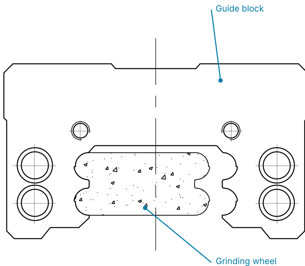
Grinding wheel and guide block in profile contact
