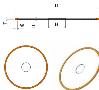
1A1R: section, dimension codes and tool model
