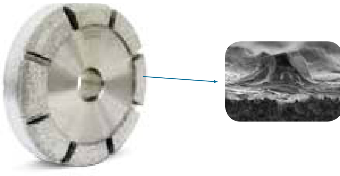
BSL: grinding wheel and abrasive-layer detail.
