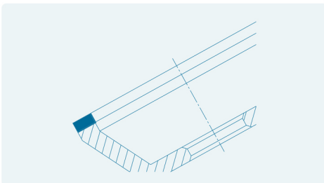
Tool cross-sections: body and grinding layer
