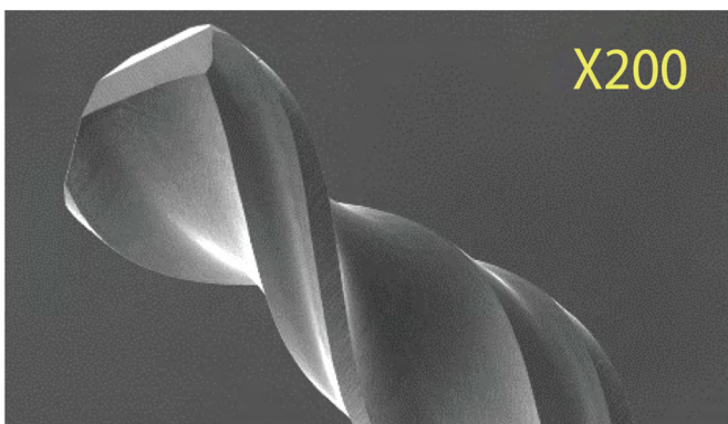
Micro cutting tool, ×200
