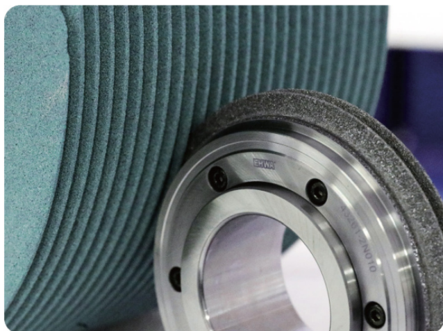
Rotary dresser in the gear-grinding process
