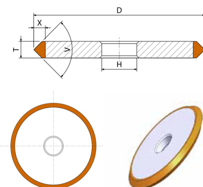
1E1: section, dimension codes and tool model
