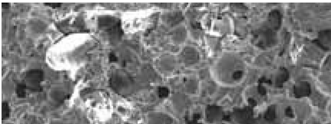
Porous hybrid bond: microstructure
