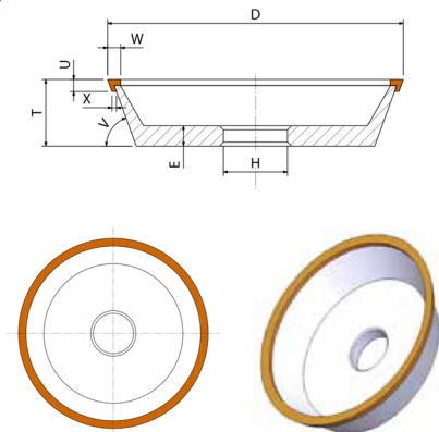
11Y9: section, dimension codes and tool model
