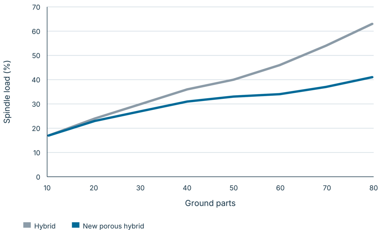
Spindle load versus ground parts: hybrid and new porous hybrid bond
