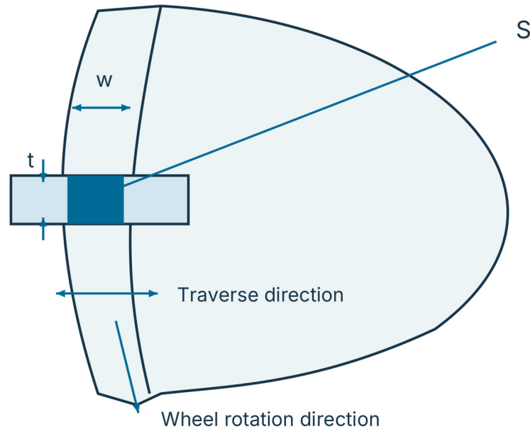
Contact area S , layer width w and contact length t
