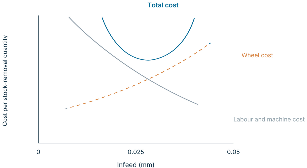
Schematic processing cost versus infeed
