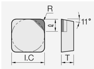
SPGN (PCD / CVD): insert dimension drawing with the corresponding geometry symbols.
