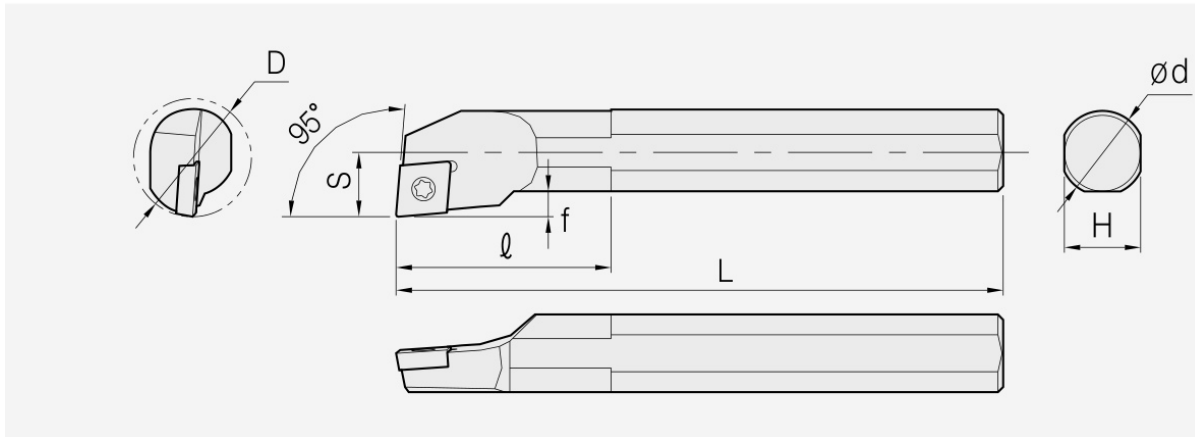
SCLC: holder dimension drawing; item dimensions and spare parts are listed in the corresponding tables.
