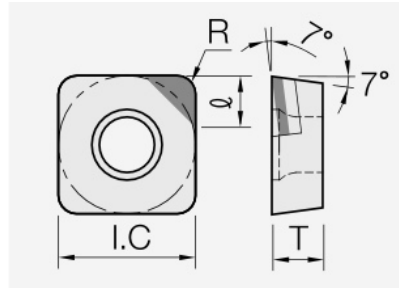
SCGT (PCD / CVD): insert dimension drawing with the corresponding geometry symbols.
