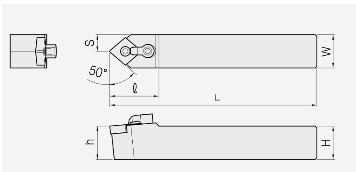
MCMNN: holder dimension drawing; item dimensions and spare parts are listed in the corresponding tables.
