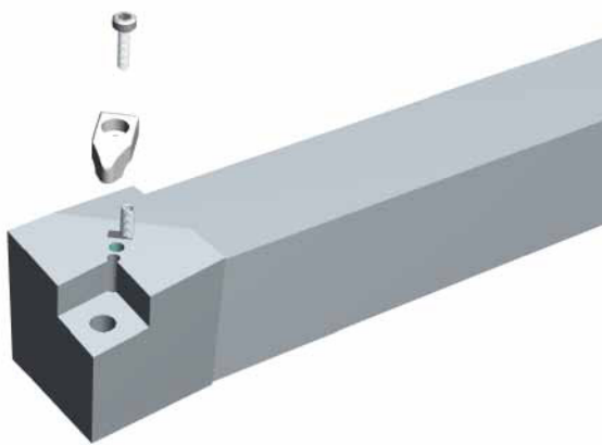
Double and lever clamping: assembly: Tool view.
