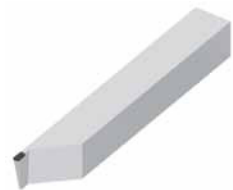
Custom tools for facing, grooving, chamfering and profiling: Tool view.
