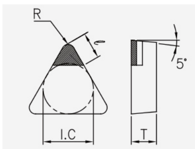
TBGN (PCD / CVD): insert dimension drawing with the corresponding geometry symbols.
