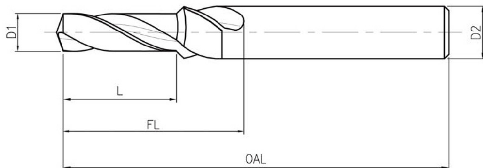
Helical drill: dimension scheme D1, D2, L, FL and OAL.
