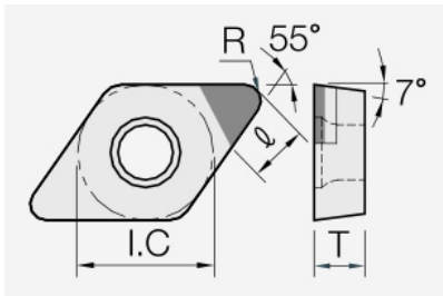
DCGW (PCBN): insert dimension drawing with the corresponding geometry symbols.
