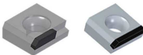
AF, BF, CF and XF face milling cutters: Tool view.
