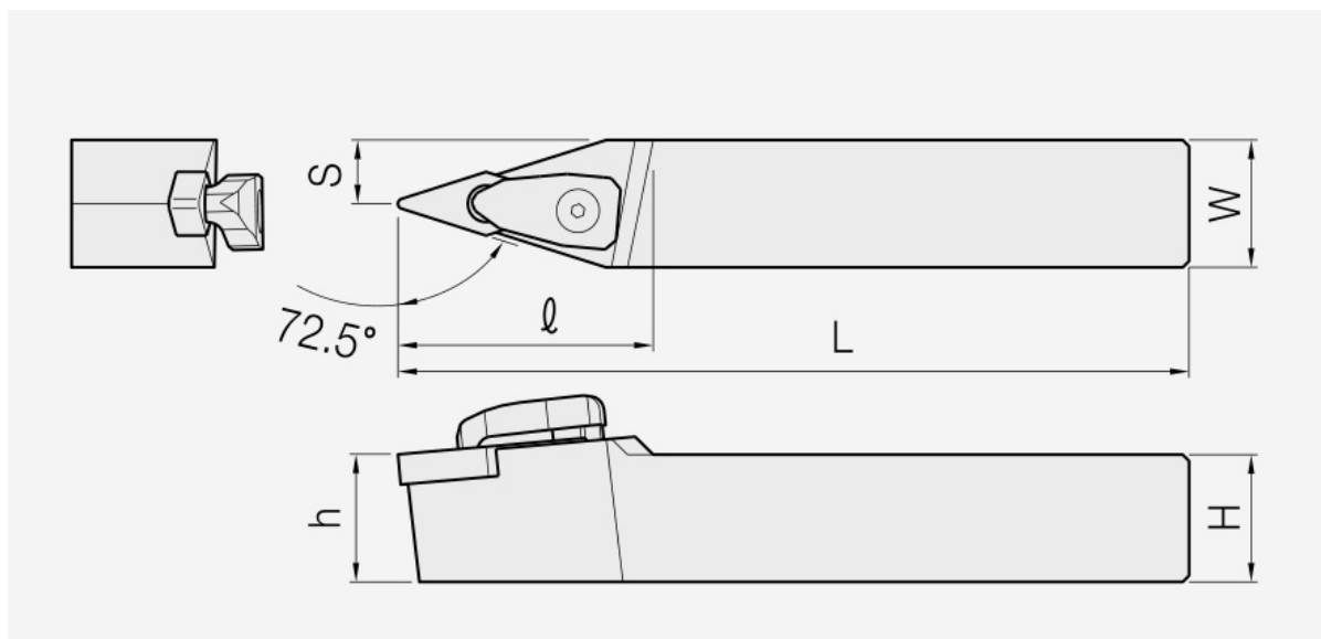
DVWNN: holder dimension drawing; item dimensions and spare parts are listed in the corresponding tables.
