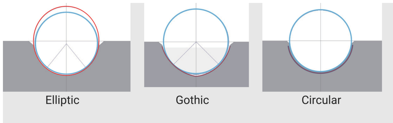
Elliptic, gothic and circular ball-track profiles.
