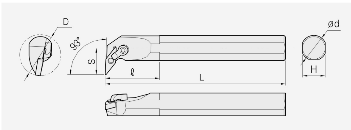
MVUN: holder dimension drawing; item dimensions and spare parts are listed in the corresponding tables.
