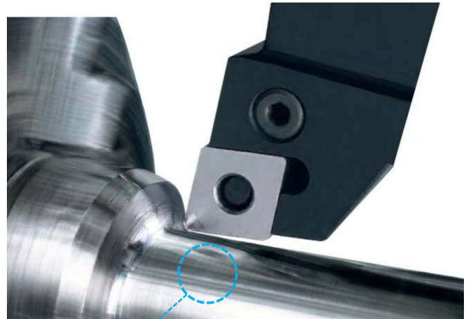
Illustrative machining view with a wiper.
