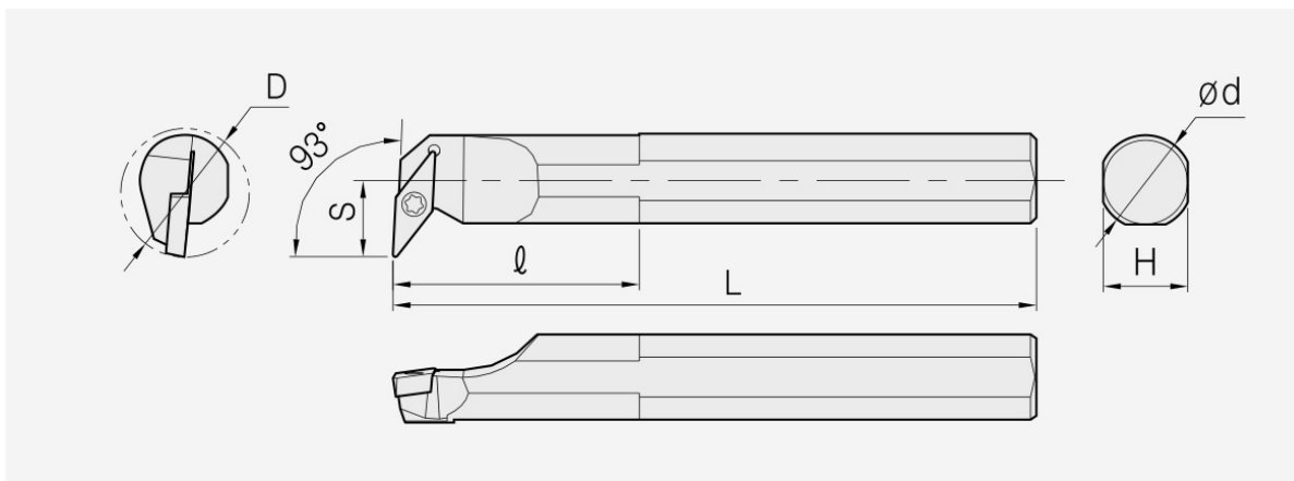
SVUB: holder dimension drawing; item dimensions and spare parts are listed in the corresponding tables.
