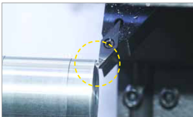
PCD chipbreakers: aluminium application examples: Component and machining view.
