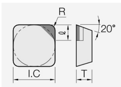
SEGN (PCD / CVD): insert dimension drawing with the corresponding geometry symbols.
