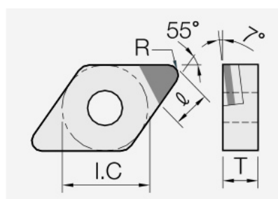
DNGX (PCD / CVD): insert dimension drawing with the corresponding geometry symbols.
