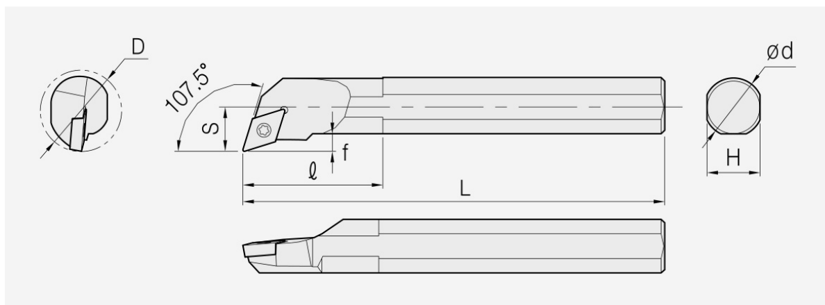
SDQC: holder dimension drawing; item dimensions and spare parts are listed in the corresponding tables.
