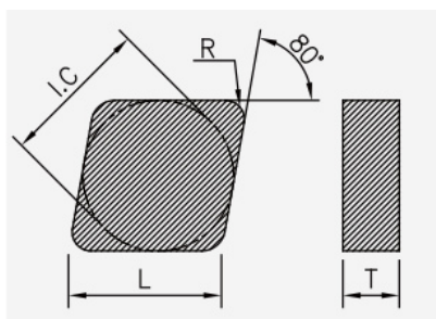
CNGN (solid) (PCBN): insert dimension drawing with the corresponding geometry symbols.
