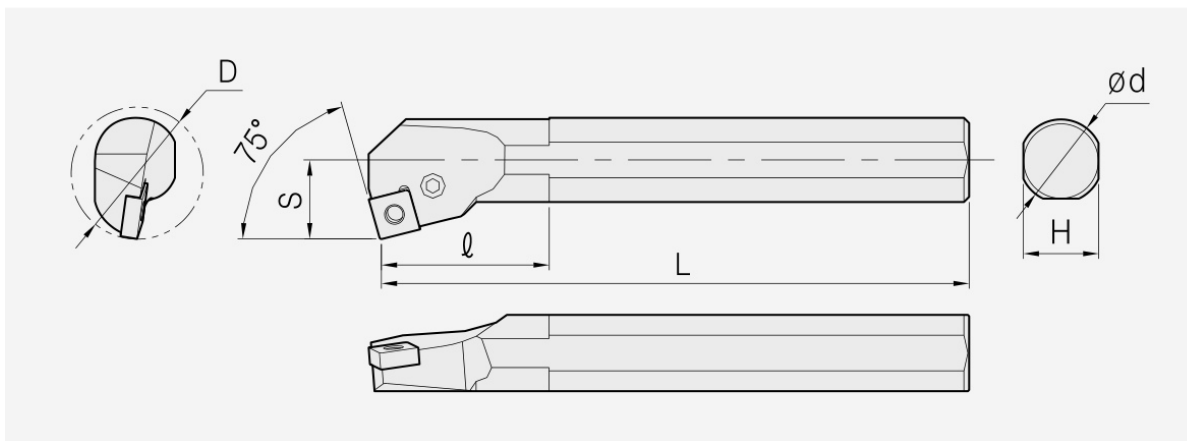
PSKN: holder dimension drawing; item dimensions and spare parts are listed in the corresponding tables.
