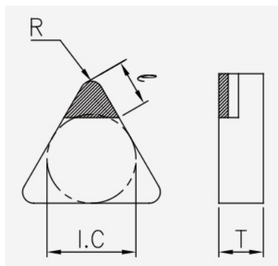
TNGN (PCBN): insert dimension drawing with the corresponding geometry symbols.
