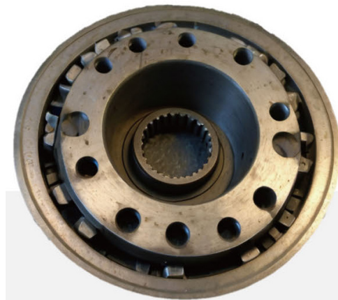
EB319: coated PCBN for hardened steel: Component and machining view.
