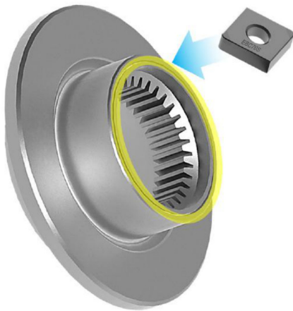
Machining position on the spline-gear test component.
