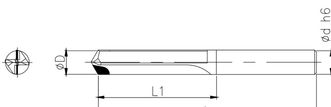
Tool: isolated dimensioned drawing; views and dimension references unchanged.
