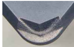
PCBN chipbreakers: SCM420 application examples: Tool view.
