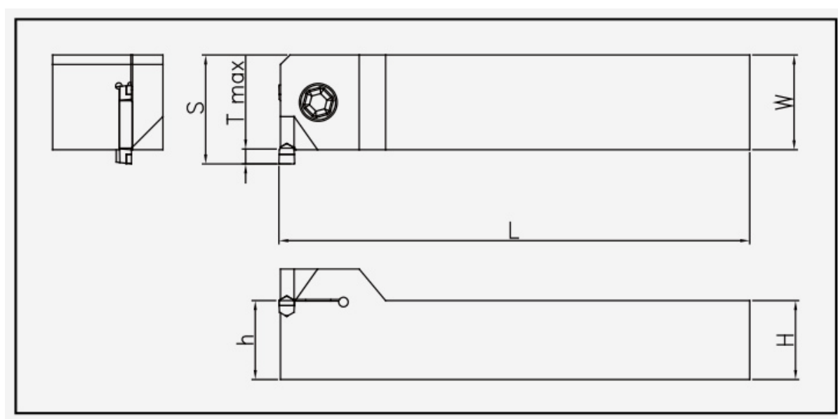
ESEV: holder dimension drawing; item dimensions and spare parts are listed in the corresponding tables.
