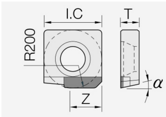
Insert: isolated dimensioned drawing with unchanged geometry symbols.
