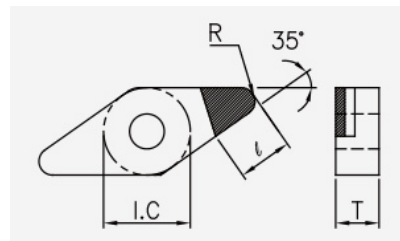
VNGA (PCD / CVD): insert dimension drawing with the corresponding geometry symbols.
