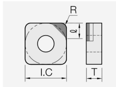
SNGA (PCBN): insert dimension drawing with the corresponding geometry symbols.
