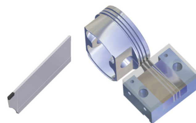
Grooving, parting, whirling and pistons: Component and machining view.
