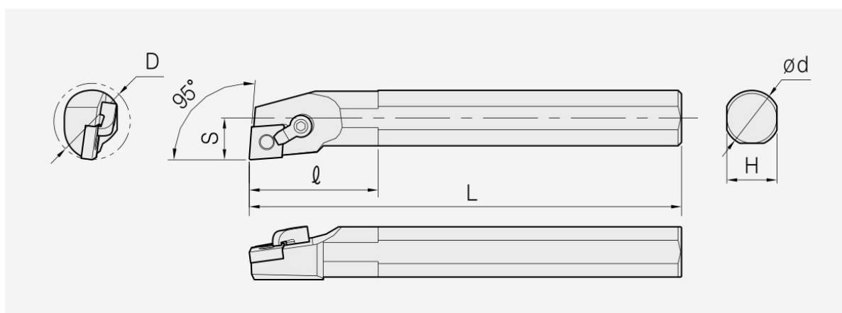
MCLN: holder dimension drawing; item dimensions and spare parts are listed in the corresponding tables.
