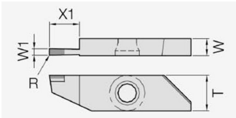
EMG type: isolated dimension scheme.
