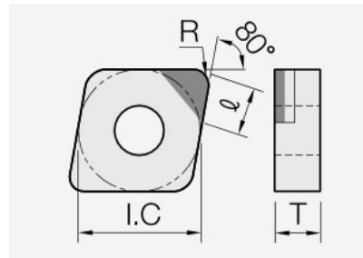
CNGA (PCD / CVD): insert dimension drawing with the corresponding geometry symbols.
