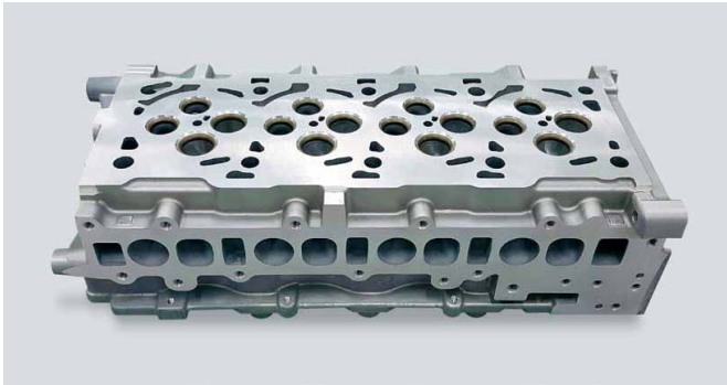
Aluminium cylinder head: valve areas and faces: Component and machining view.
