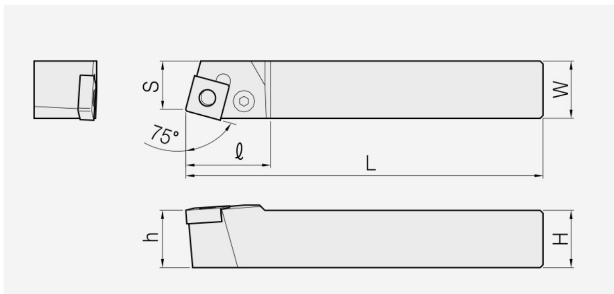
Tool: isolated dimensioned drawing; views and dimension references unchanged.
