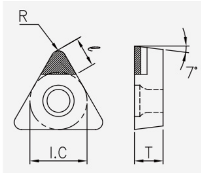
TCGW (PCBN): insert dimension drawing with the corresponding geometry symbols.
