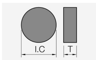
RNGN (solid) (PCBN): insert dimension drawing with the corresponding geometry symbols.
