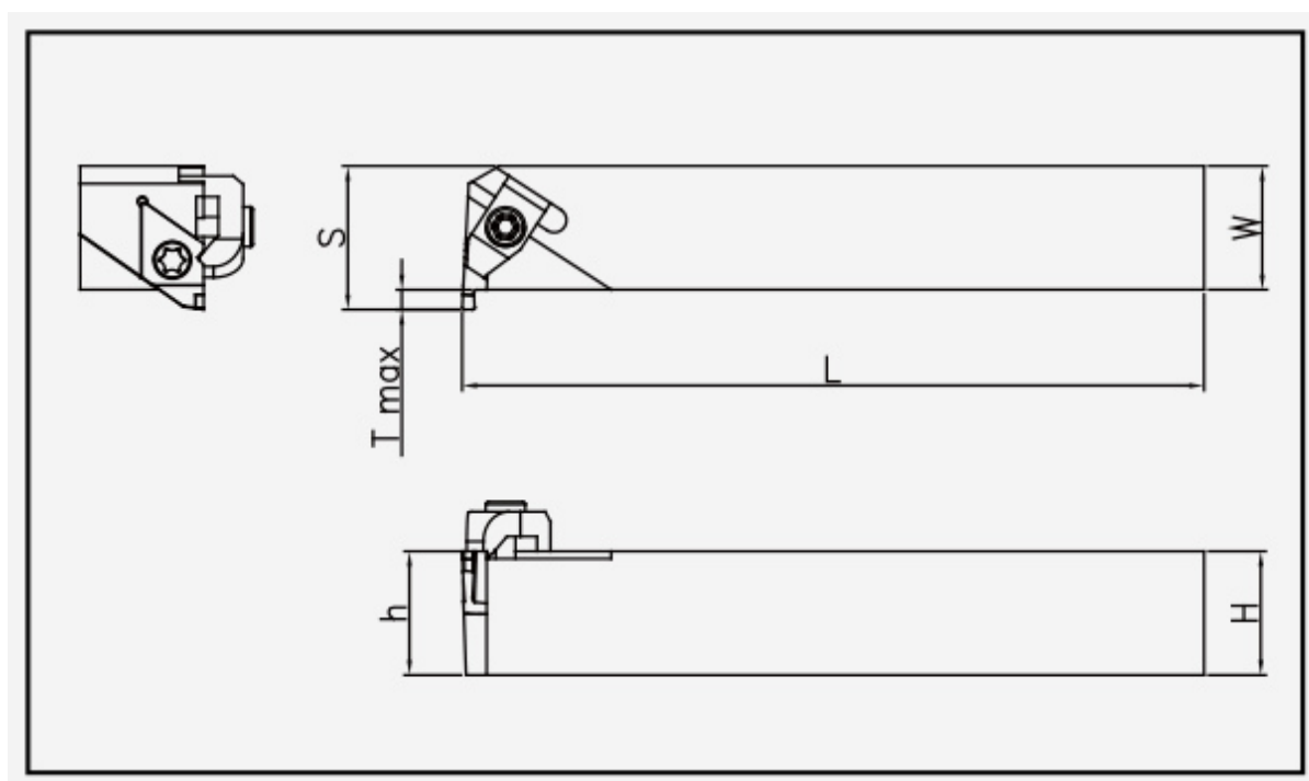
EDEV: holder dimension drawing; item dimensions and spare parts are listed in the corresponding tables.
