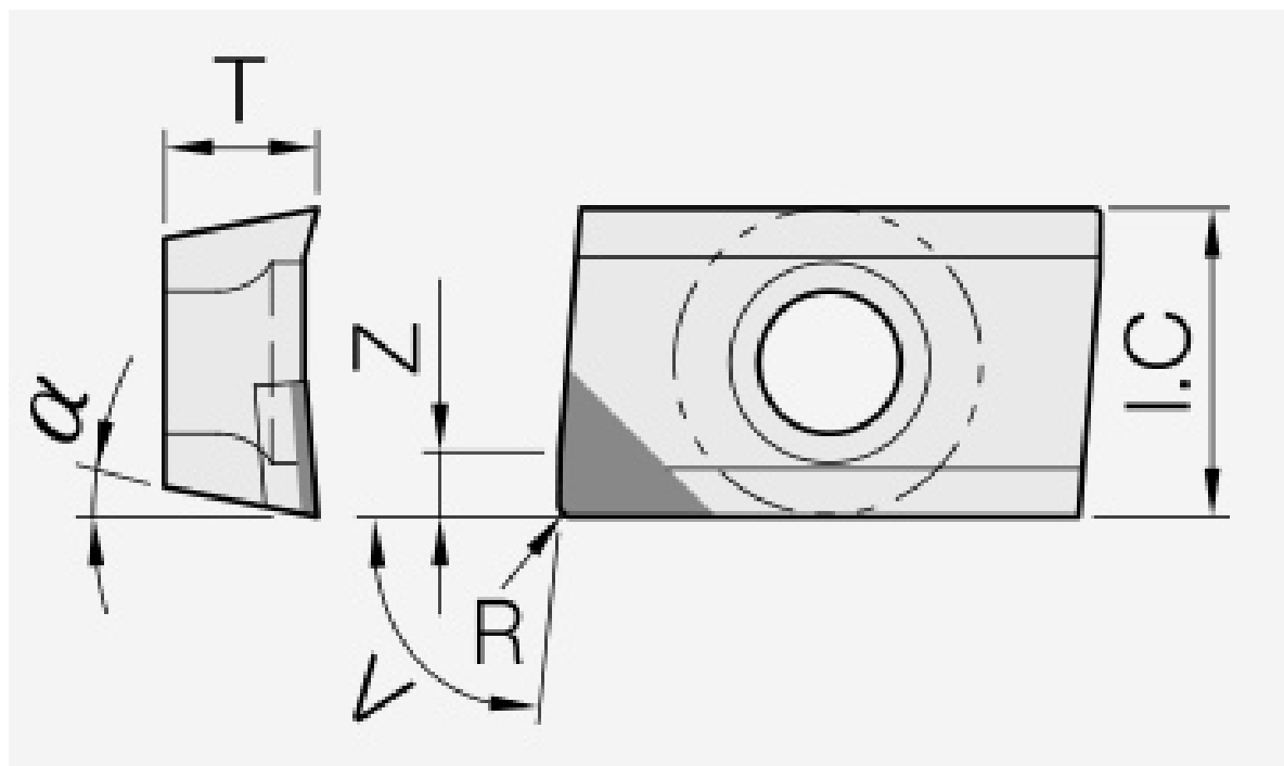
Insert: isolated dimensioned drawing with unchanged geometry symbols.
