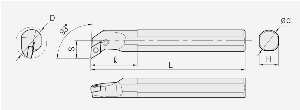
PDUN: holder dimension drawing; item dimensions and spare parts are listed in the corresponding tables.
