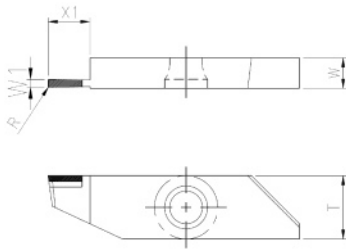
EMG: dimensional drawing.
