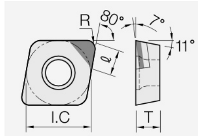
CPGT (PCD / CVD): insert dimension drawing with the corresponding geometry symbols.
