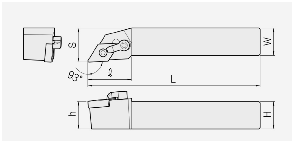
MDJN: holder dimension drawing; item dimensions and spare parts are listed in the corresponding tables.
