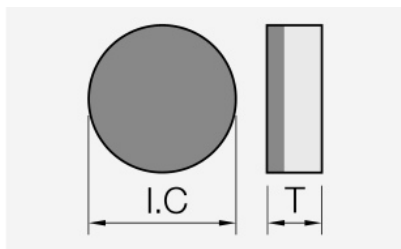
RNGN (PCD / CVD): insert dimension drawing with the corresponding geometry symbols.
