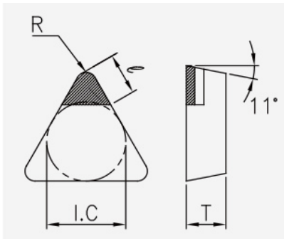
TPGN (PCD / CVD): insert dimension drawing with the corresponding geometry symbols.
