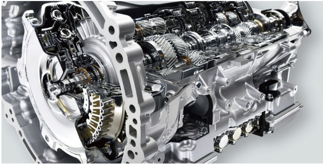
EB319: coated PCBN for hardened steel: Component and machining view.
