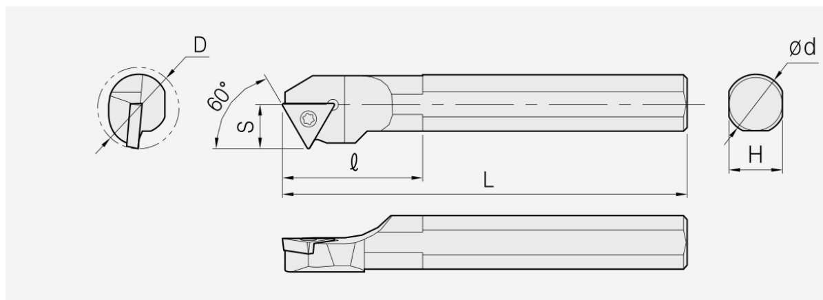
STWP: holder dimension drawing; item dimensions and spare parts are listed in the corresponding tables.
