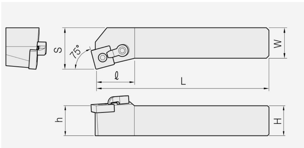
MSKN: holder dimension drawing; item dimensions and spare parts are listed in the corresponding tables.
