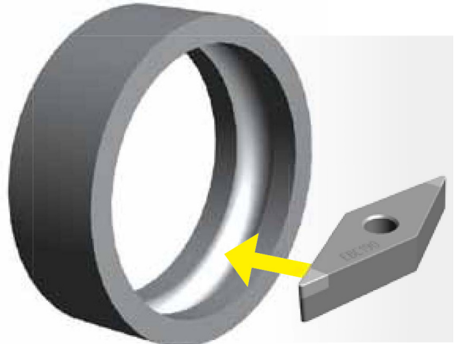
EBC190: coated PCBN for hardened workpieces: Component and machining view.
