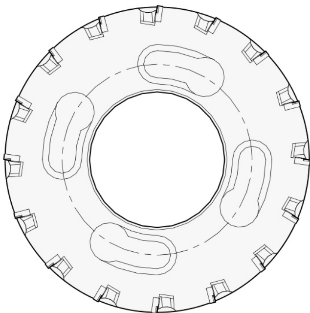
Steel cutter bodies and PCBN inserts: Tool view.
