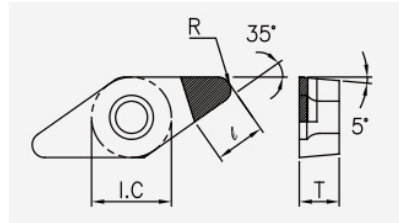
VBGW (PCBN): insert dimension drawing with the corresponding geometry symbols.
