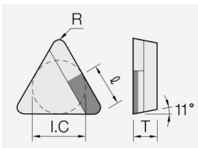
TPGN (R) (PCD / CVD): insert dimension drawing with the corresponding geometry symbols.
