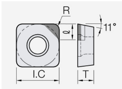
SPGW (PCD / CVD): insert dimension drawing with the corresponding geometry symbols.
