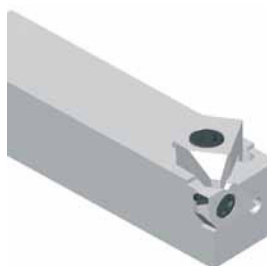
Custom inserts and holder examples: Tool view.
