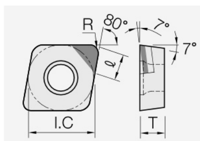
CCGT (PCD / CVD): insert dimension drawing with the corresponding geometry symbols.
