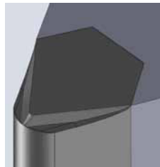
PCBN chipbreakers ER, EF and ES: Tool view.
