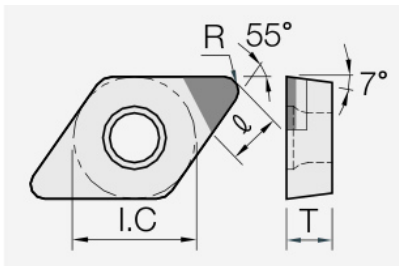
DCGW (PCD / CVD): insert dimension drawing with the corresponding geometry symbols.
