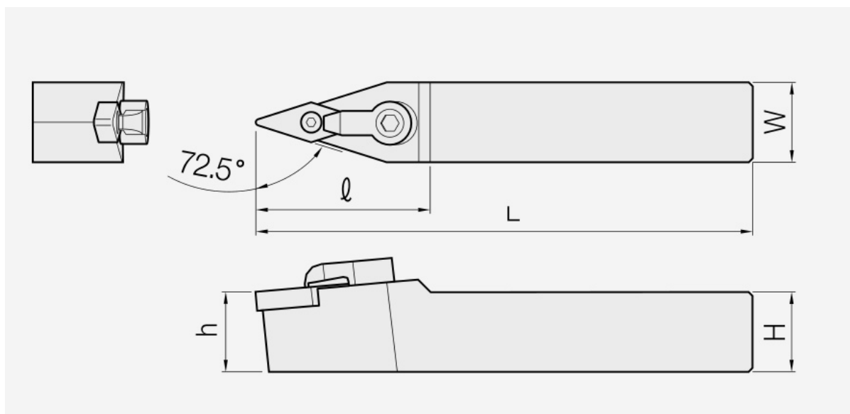
MVWNN: holder dimension drawing; item dimensions and spare parts are listed in the corresponding tables.
