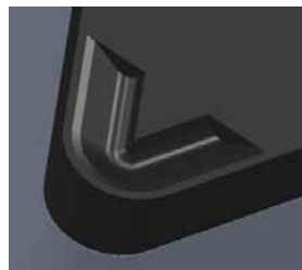
PCD/CVD chipbreakers ER and EX: Tool view.
