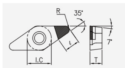
VCGW (PCBN): insert dimension drawing with the corresponding geometry symbols.
