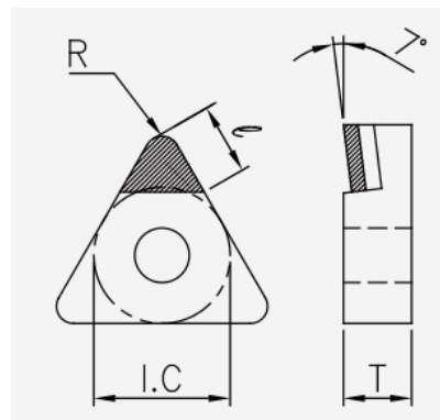
TNGX (PCD / CVD): insert dimension drawing with the corresponding geometry symbols.
