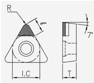
TCGW (PCD / CVD): insert dimension drawing with the corresponding geometry symbols.
