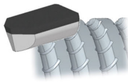
PCD grades EP20, EP55 and EP59: Component and machining view.
