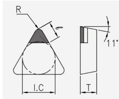
TPGN (PCBN): insert dimension drawing with the corresponding geometry symbols.
