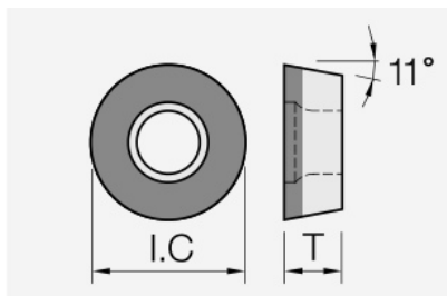
RPGW (PCD / CVD): insert dimension drawing with the corresponding geometry symbols.
