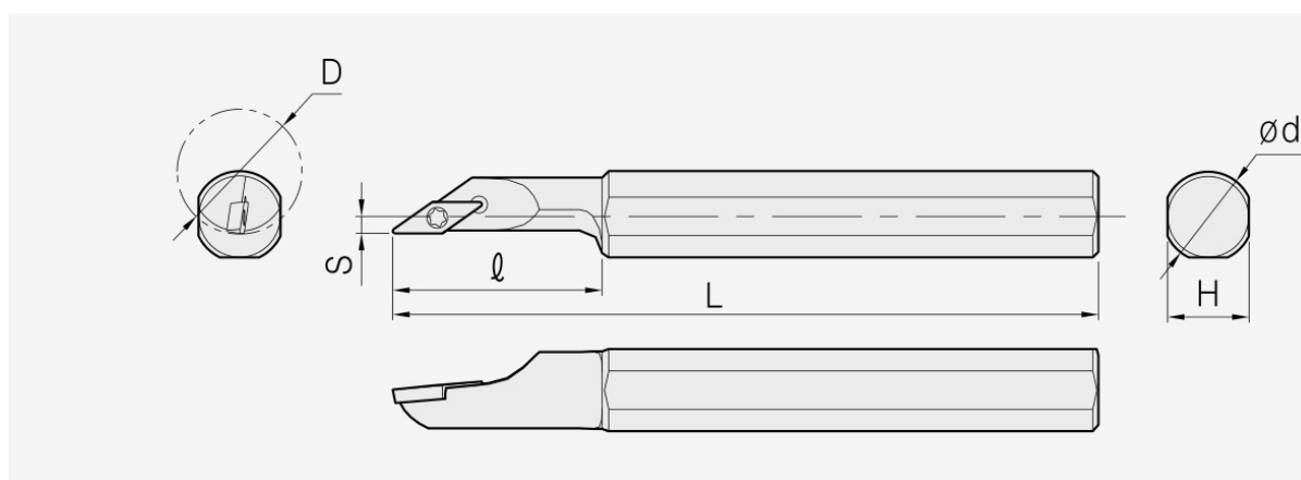
SVJC: holder dimension drawing; item dimensions and spare parts are listed in the corresponding tables.
