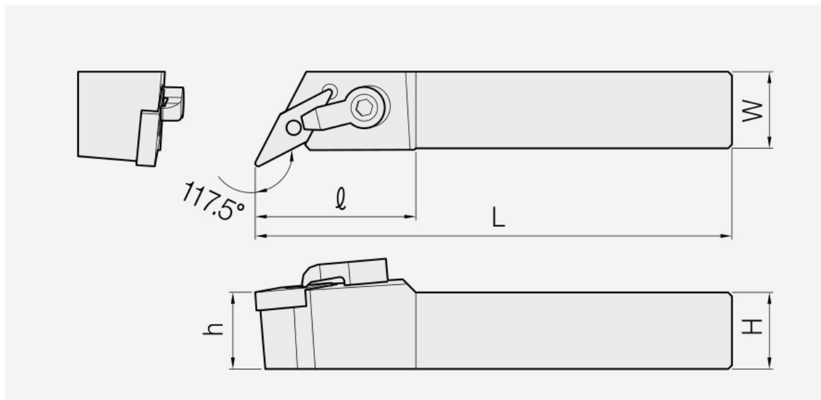
MVQN: holder dimension drawing; item dimensions and spare parts are listed in the corresponding tables.
