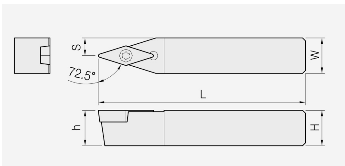
SVVBN: holder dimension drawing; item dimensions and spare parts are listed in the corresponding tables.
