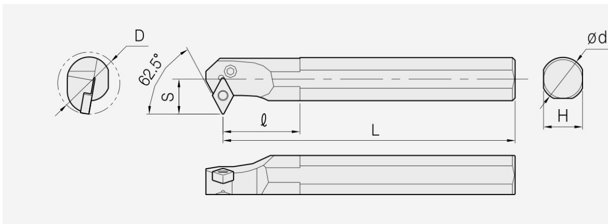
PDSN: holder dimension drawing; item dimensions and spare parts are listed in the corresponding tables.
