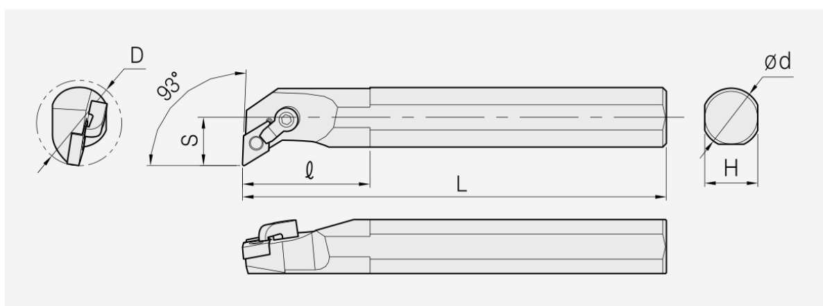
MDUN: holder dimension drawing; item dimensions and spare parts are listed in the corresponding tables.
