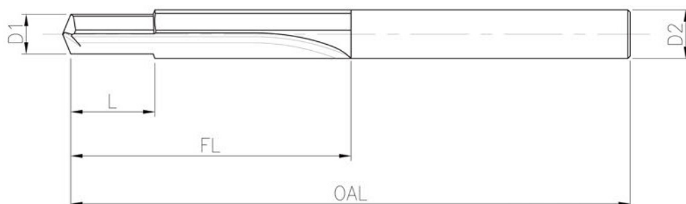
Burnishing drill: dimension scheme D1, D2, L, FL and OAL.
