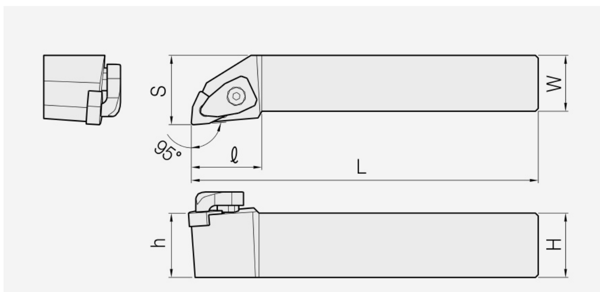
DWLN: holder dimension drawing; item dimensions and spare parts are listed in the corresponding tables.
