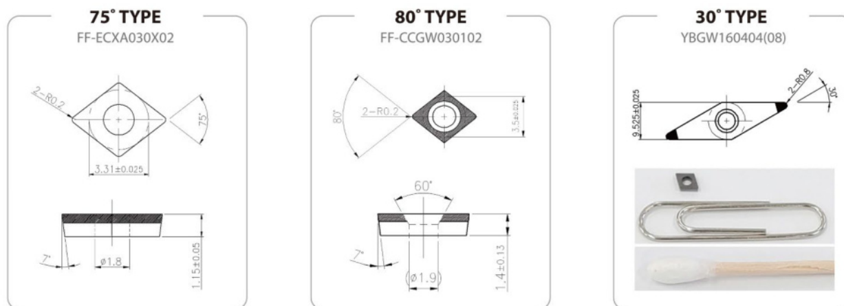
Micro geometries with the complete dimensional and tolerance annotations.
