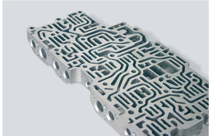
Aluminium-alloy valve bodies: Component and machining view.
