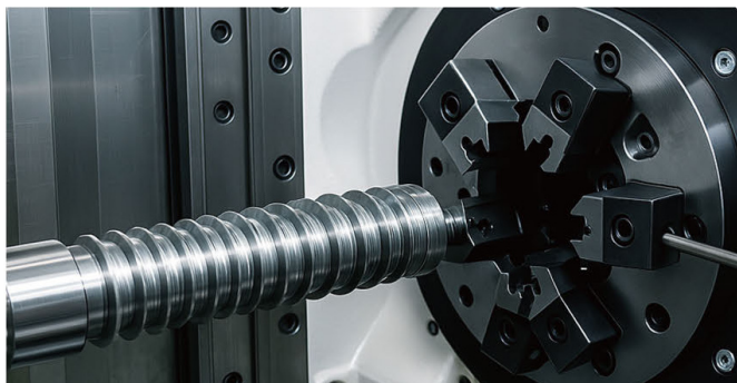
Whirling: geometry, grades and coatings: Component and machining view.
