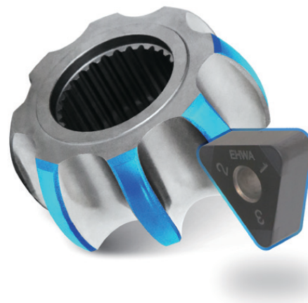
Inner-race hard turning.
