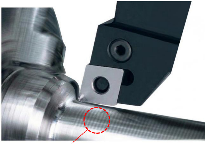
Illustrative machining view without a wiper.
