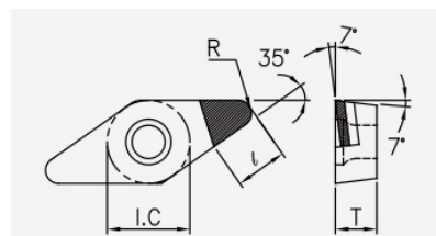
VCGT (PCD / CVD): insert dimension drawing with the corresponding geometry symbols.
