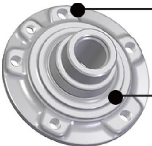
Bearings: internal turning and drilling: Component and machining view.
