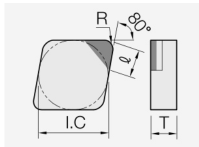
CNGN (PCBN): insert dimension drawing with the corresponding geometry symbols.
