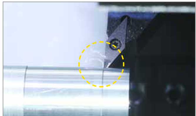
PCD chipbreakers: aluminium application examples: Component and machining view.
