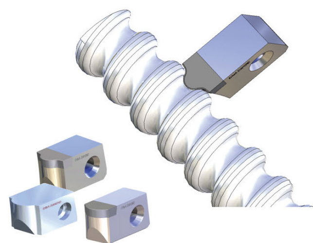
Grooving, parting, whirling and pistons: Tool view.
