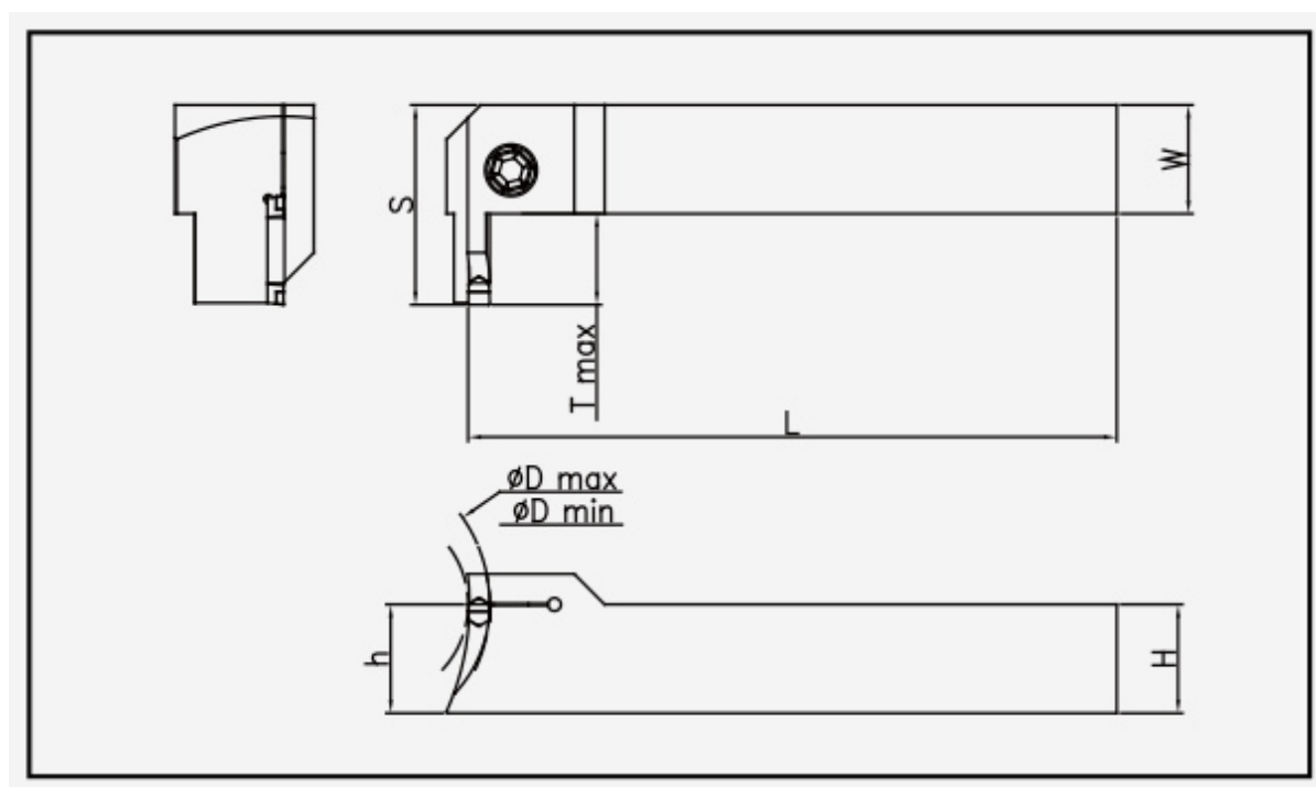
ESFV: holder dimension drawing; item dimensions and spare parts are listed in the corresponding tables.
