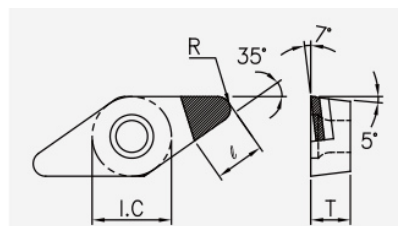
VBGT (PCD / CVD): insert dimension drawing with the corresponding geometry symbols.
