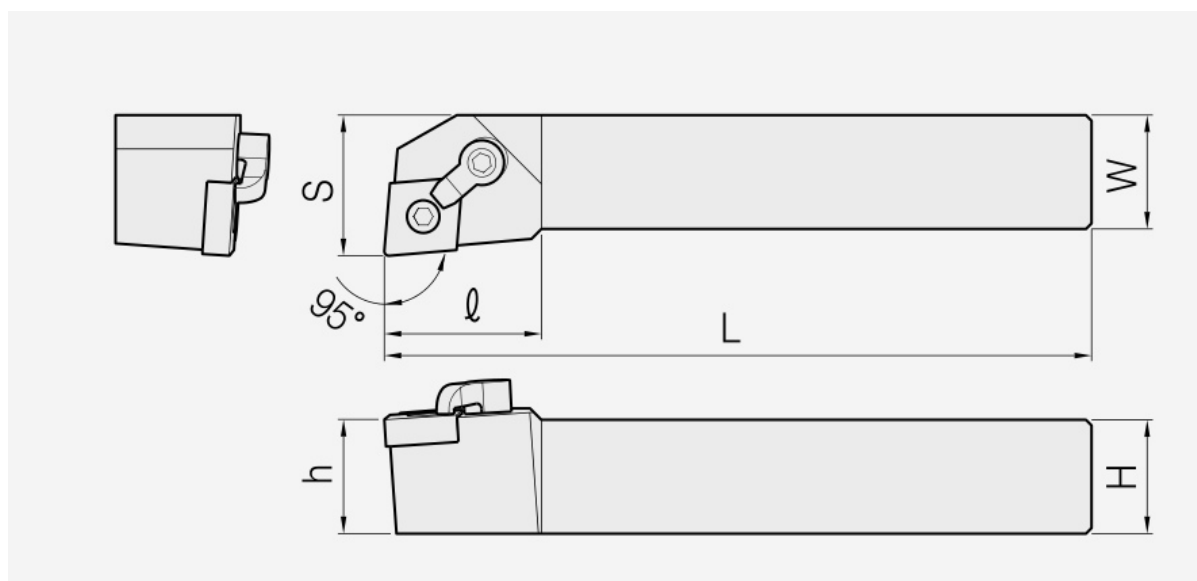
MCLN: holder dimension drawing; item dimensions and spare parts are listed in the corresponding tables.
