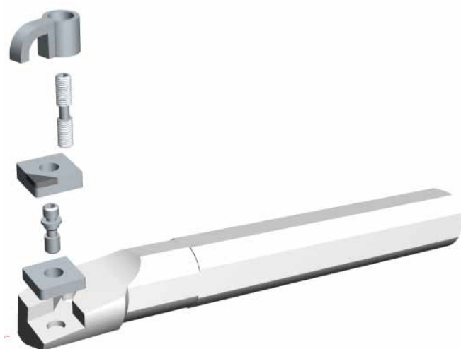
Boring holders: double clamping and multi locking: Tool view.
