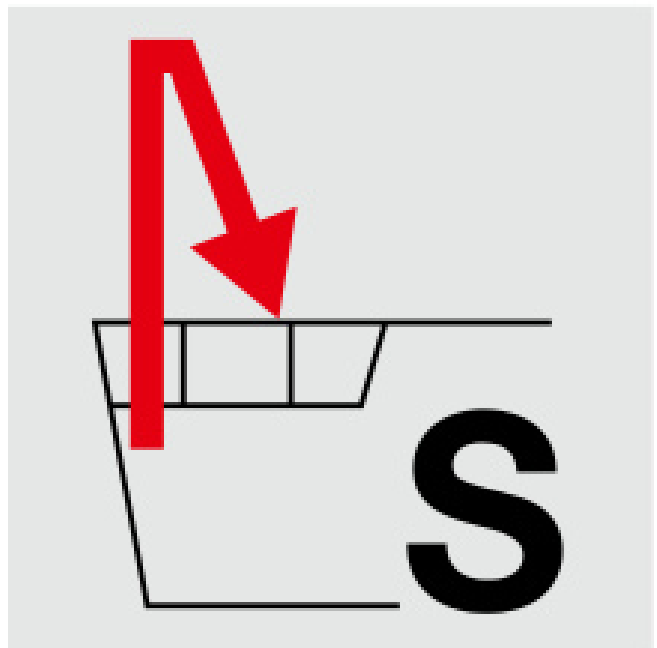
Clamping principle S: unchanged arrow directions.
