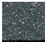
PCD: grain size, diamond content and grade selection: Microstructure image with the shown scale.
