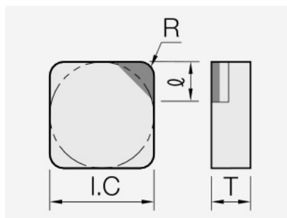
SNGN (PCBN): insert dimension drawing with the corresponding geometry symbols.
