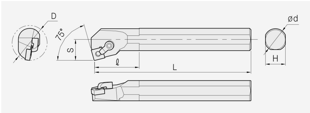
MSKN: holder dimension drawing; item dimensions and spare parts are listed in the corresponding tables.
