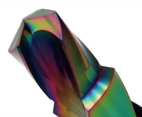
Solid carbide drills and coatings: Tool view.
