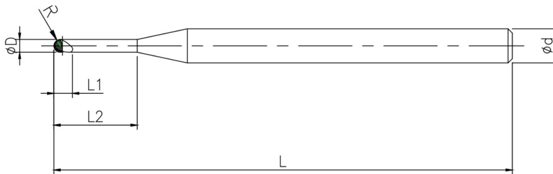
EBEB: PCBN ball-nose end mills: Tool view.
