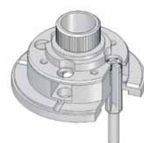
Gears and clutch: Component and machining view.
