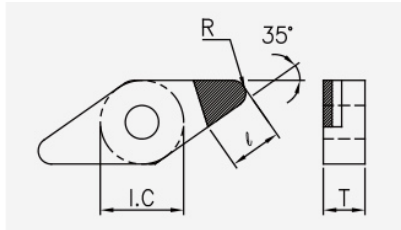
VNGA (PCBN): insert dimension drawing with the corresponding geometry symbols.
