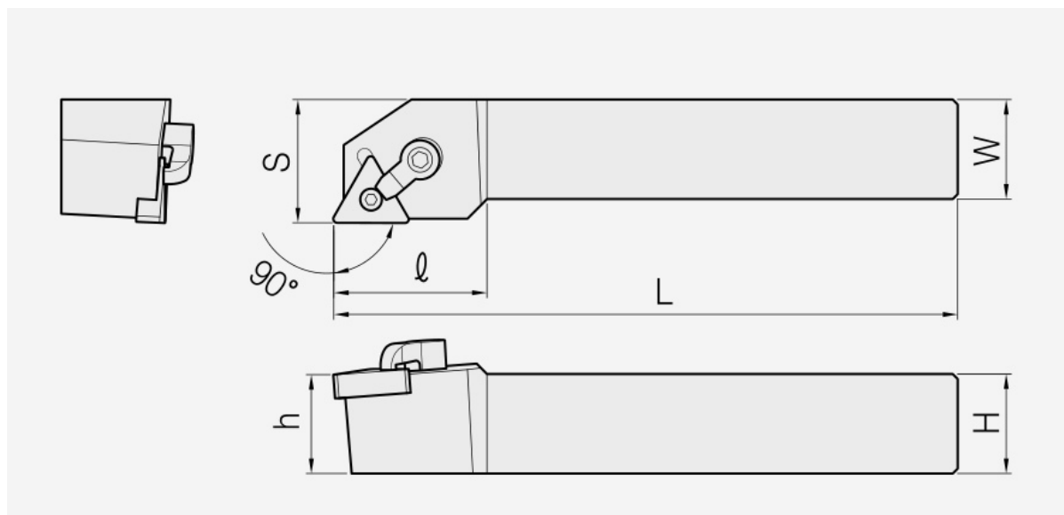
MTGN: holder dimension drawing; item dimensions and spare parts are listed in the corresponding tables.
