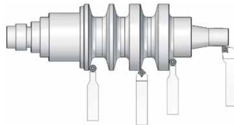
Steel-roll machining: Tool view.
