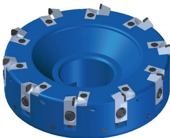
AF, BF, CF and XF face milling cutters: Tool view.
