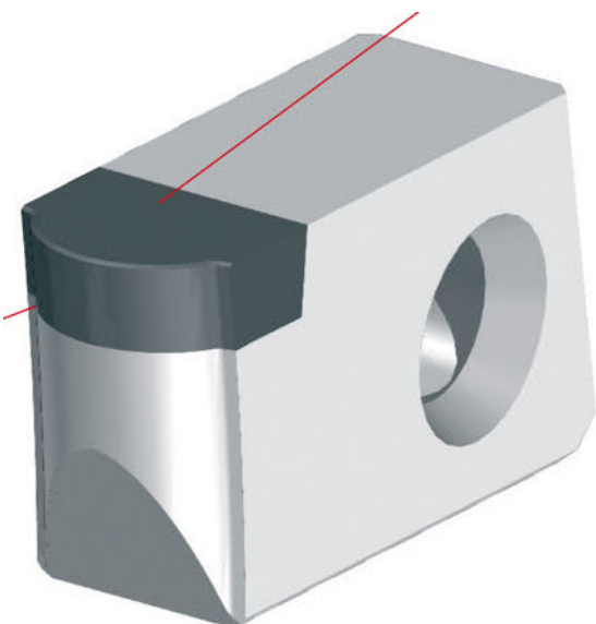
Whirling: geometry, grades and coatings: Tool view.
