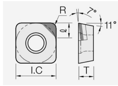
SPGT (PCD / CVD): insert dimension drawing with the corresponding geometry symbols.
