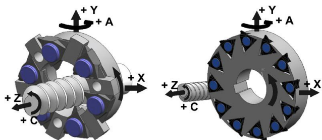
EB12 whirling tools with axis illustration.
