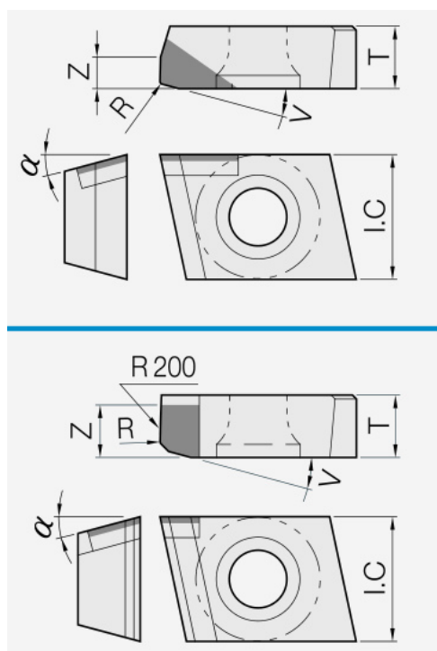
Insert: isolated dimensioned drawing with unchanged geometry symbols.
