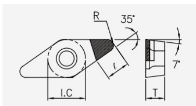
VCGW (PCD / CVD): insert dimension drawing with the corresponding geometry symbols.
