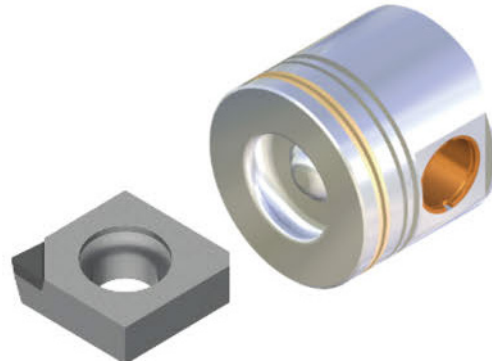
PCD grades EP20, EP55 and EP59: Component and machining view.
