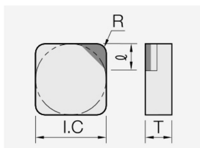
SNGN (PCD / CVD): insert dimension drawing with the corresponding geometry symbols.
