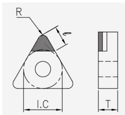
TNGA (PCBN): insert dimension drawing with the corresponding geometry symbols.
