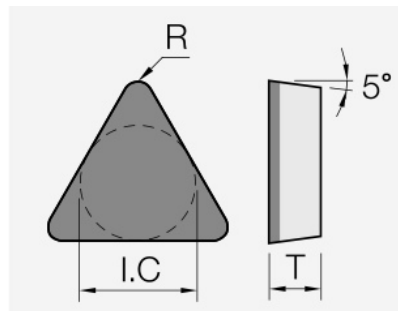
TBGN (PCBN): insert dimension drawing with the corresponding geometry symbols.
