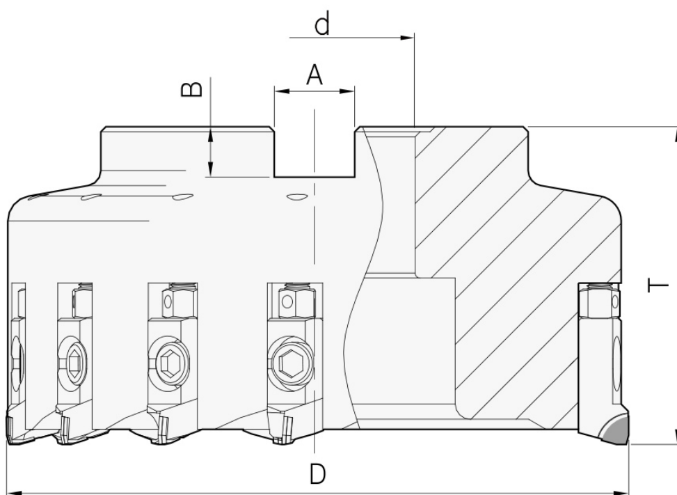
Tool: isolated dimensioned drawing; views and dimension references unchanged.
