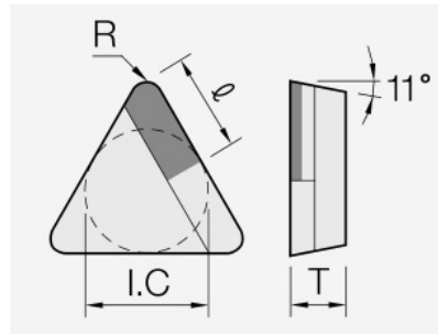
TPGN (L) (PCD / CVD): insert dimension drawing with the corresponding geometry symbols.
