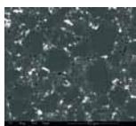
PCD: grain size, diamond content and grade selection: Microstructure image with the shown scale.
