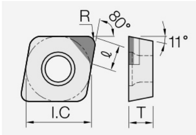
CPGW (PCD / CVD): insert dimension drawing with the corresponding geometry symbols.
