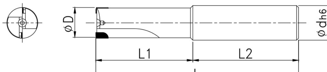
Tool: isolated dimensioned drawing; views and dimension references unchanged.
