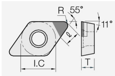
DPGW (PCD / CVD): insert dimension drawing with the corresponding geometry symbols.
