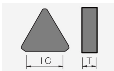
TNGN (solid) (PCBN): insert dimension drawing with the corresponding geometry symbols.
