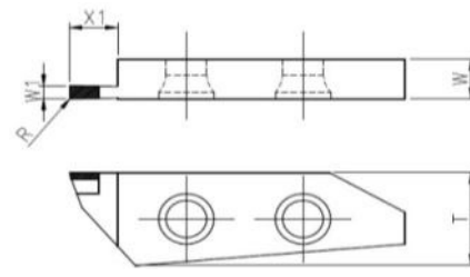
EMG2: dimensional drawing.
