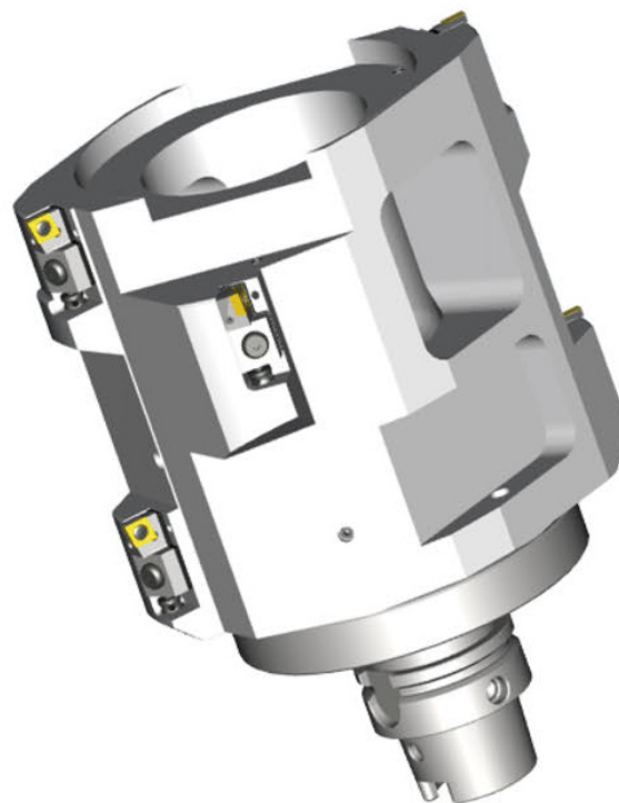
Special boring tool for motor housings: Tool view.
