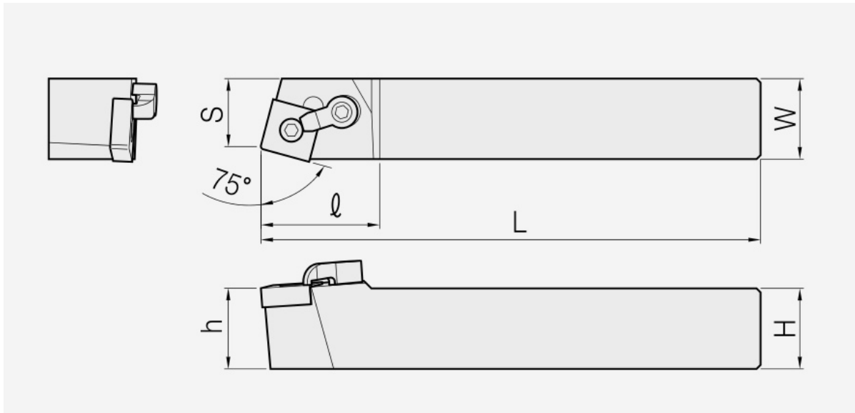
MSBN: holder dimension drawing; item dimensions and spare parts are listed in the corresponding tables.
