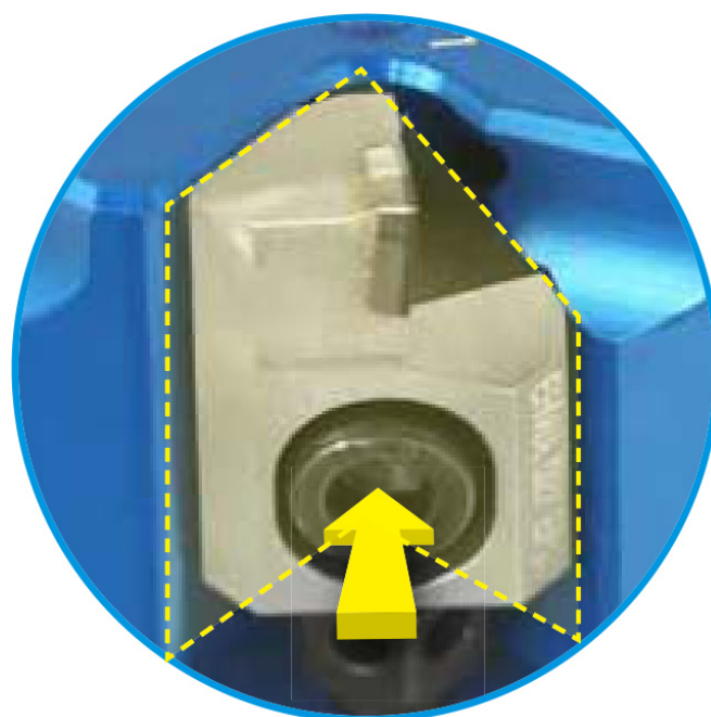
CF: cutter with directed chip and coolant flow: Component and machining view.
