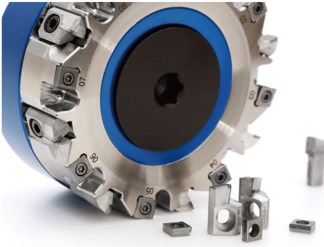
XF face milling cutters for aluminium alloys: Tool view.
