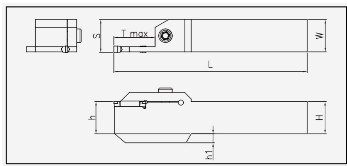
ESEH: holder dimension drawing; item dimensions and spare parts are listed in the corresponding tables.
