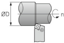
Turning: diameter D and spindle speed N in the cutting-speed model.
