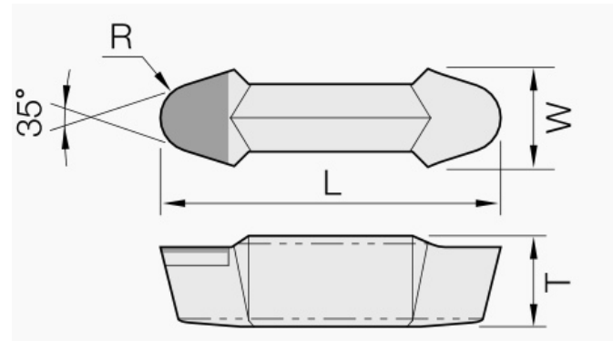
Custom shape: both tool views with their dimension references.
