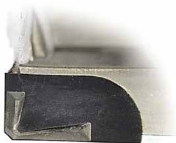
PCD reamers: standard and chip-breaker types: Tool view.
