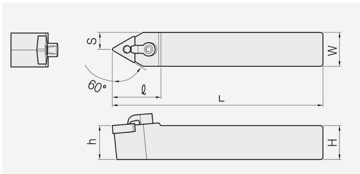
MTENN: holder dimension drawing; item dimensions and spare parts are listed in the corresponding tables.
