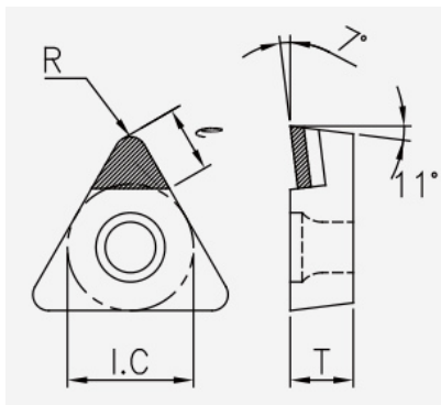
TPGT (PCD / CVD): insert dimension drawing with the corresponding geometry symbols.
