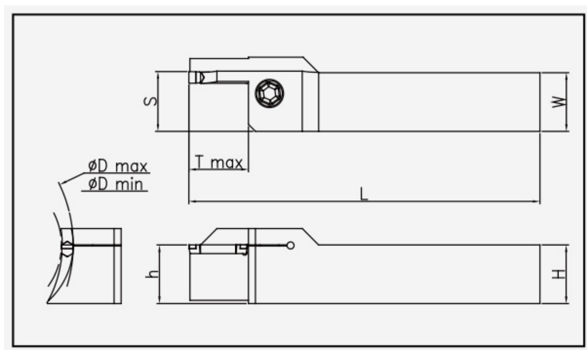
ESFH: holder dimension drawing; item dimensions and spare parts are listed in the corresponding tables.
