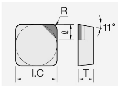
SPGN (PCBN): insert dimension drawing with the corresponding geometry symbols.
