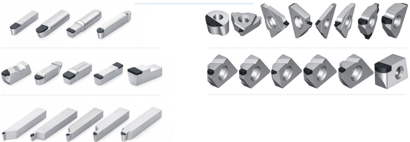
Overview of custom tool forms.
