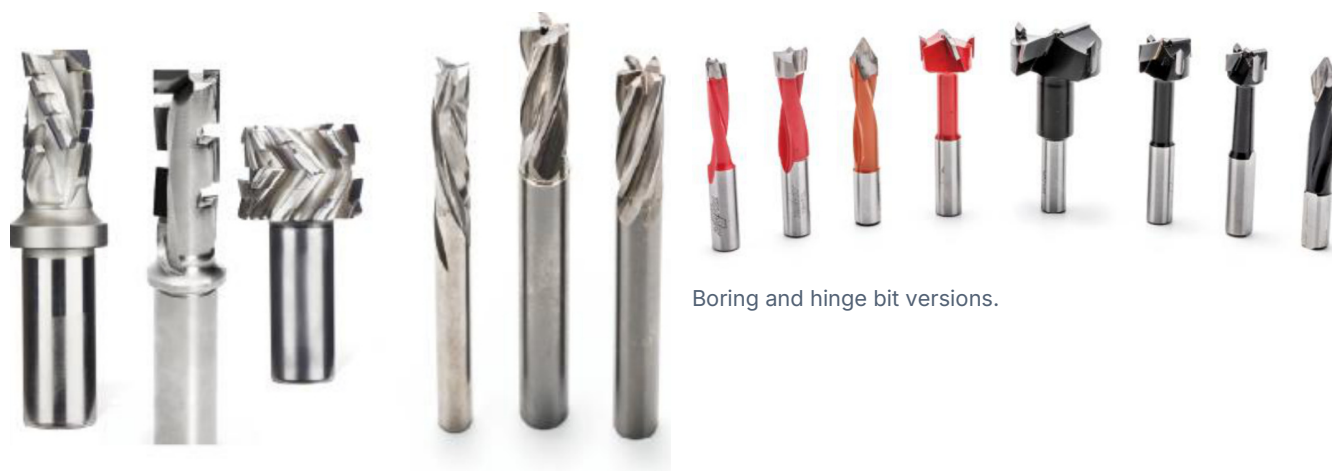
PCD/TCT router bits in different forms.
