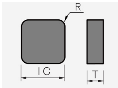
SNGN (solid) (PCBN): insert dimension drawing with the corresponding geometry symbols.
