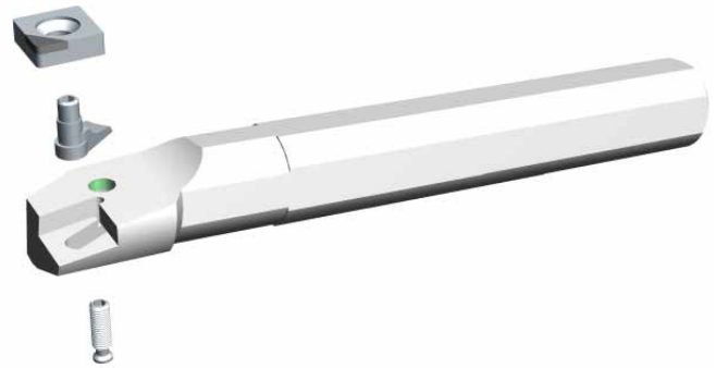
Boring holders: lever locking and screw clamping: Tool view.
