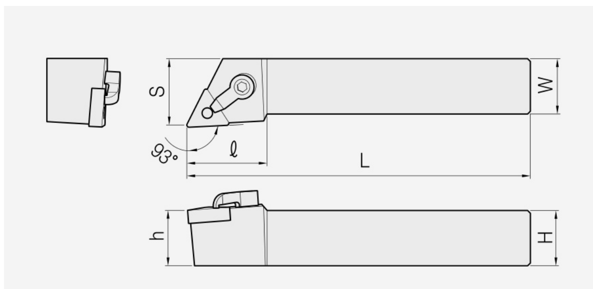
MTJN: holder dimension drawing; item dimensions and spare parts are listed in the corresponding tables.
