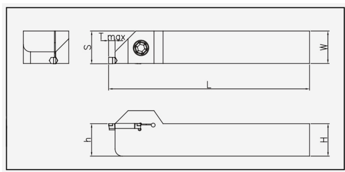
ESEH-T00: holder dimension drawing; item dimensions and spare parts are listed in the corresponding tables.
