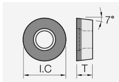
RCGW (PCD / CVD): insert dimension drawing with the corresponding geometry symbols.
