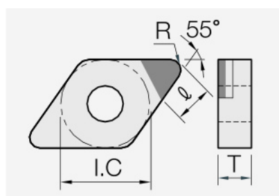
DNGA (PCD / CVD): insert dimension drawing with the corresponding geometry symbols.
