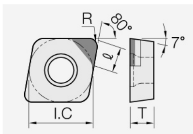
CCGW (PCBN): insert dimension drawing with the corresponding geometry symbols.
