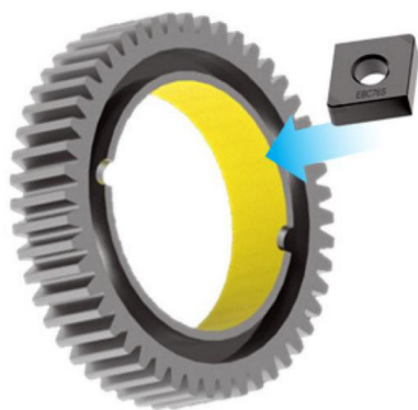
Inner machining position on the spur-gear test component.
