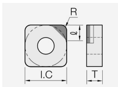
SNGA (PCD / CVD): insert dimension drawing with the corresponding geometry symbols.
