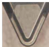
PCBN chipbreakers ER, EF and ES: Tool view.
