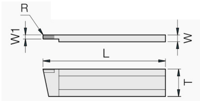
Custom shape: both tool views with their dimension references.
