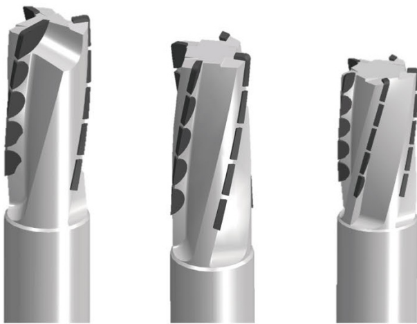
PCD end mills for electric vehicles: Tool view.
