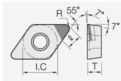
DCGT (PCD / CVD): insert dimension drawing with the corresponding geometry symbols.
