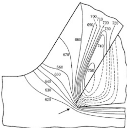
Isotherms in the source illustration; temperature labels in °C. Model image, not application-specific measurement.
