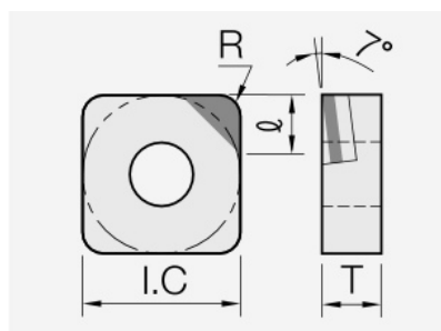
SNGX (PCD / CVD): insert dimension drawing with the corresponding geometry symbols.
