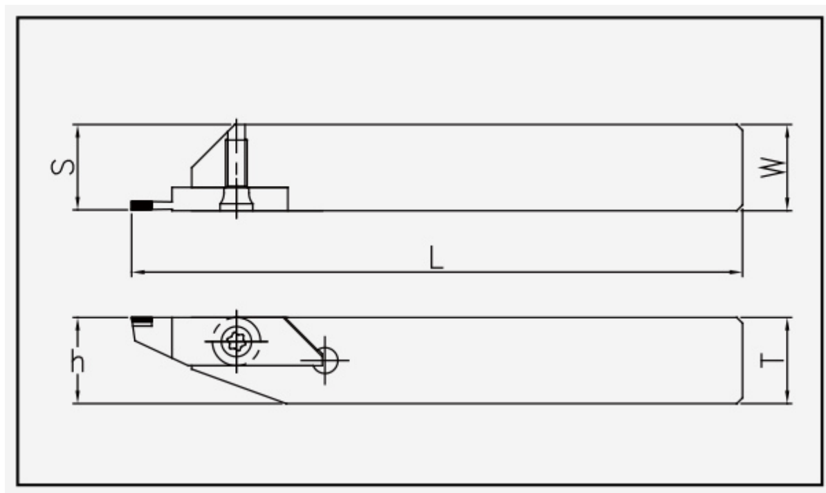
EMEH: holder dimension drawing; item dimensions and spare parts are listed in the corresponding tables.
