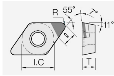
DPGT (PCD / CVD): insert dimension drawing with the corresponding geometry symbols.
