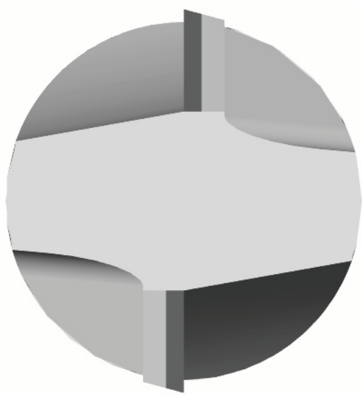
EBEB: PCBN ball-nose end mills: Tool view.
