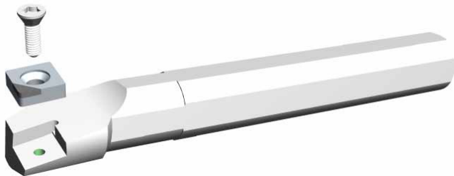
Boring holders: lever locking and screw clamping: Tool view.
