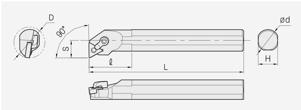
MTFN: holder dimension drawing; item dimensions and spare parts are listed in the corresponding tables.
