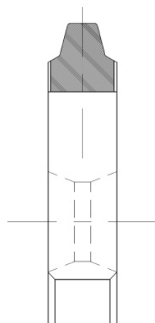
First illustrated EB12 profile form.
