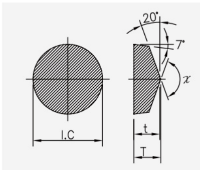
Insert: isolated dimensioned drawing with unchanged geometry symbols.
