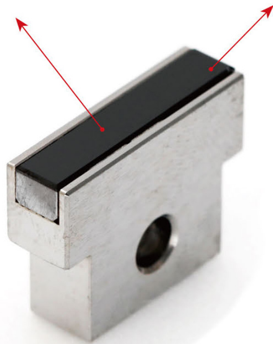
Wear parts for grinding and measuring machines: Tool view.
