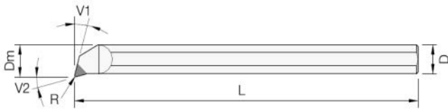
BSR/L: boring-tool dimensional drawing.
