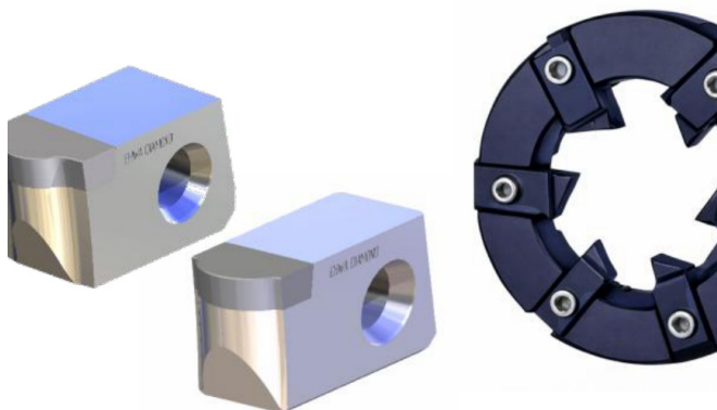
EB73 insert and whirling head.
