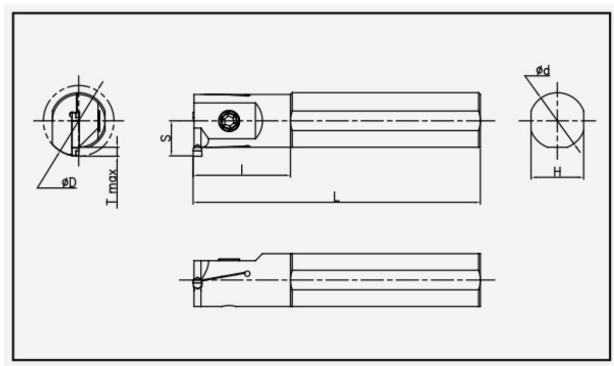
ESIV: holder dimension drawing; item dimensions and spare parts are listed in the corresponding tables.
