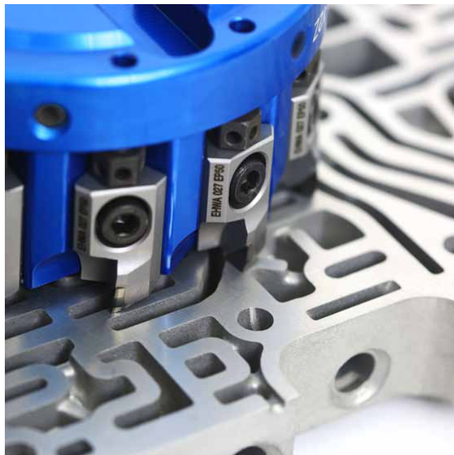
Cutting tools: complete programme: Component and machining view.
