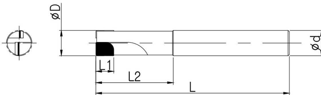
Tool: isolated dimensioned drawing; views and dimension references unchanged.
