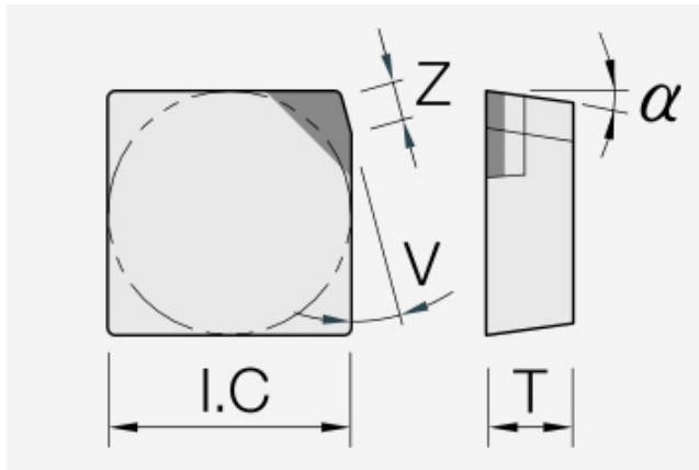
Insert: isolated dimensioned drawing with unchanged geometry symbols.
