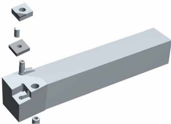
Double and lever clamping: assembly: Tool view.
