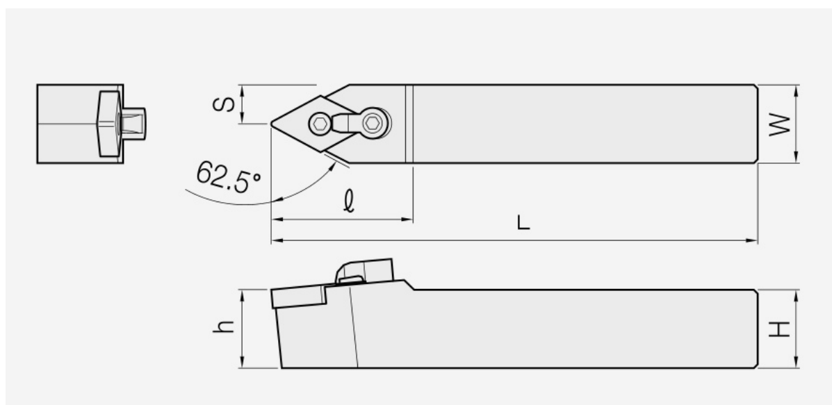
MDNNN: holder dimension drawing; item dimensions and spare parts are listed in the corresponding tables.
