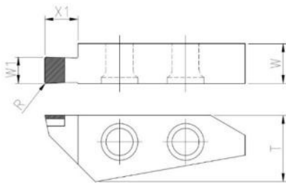
EMG3: dimensional drawing.
