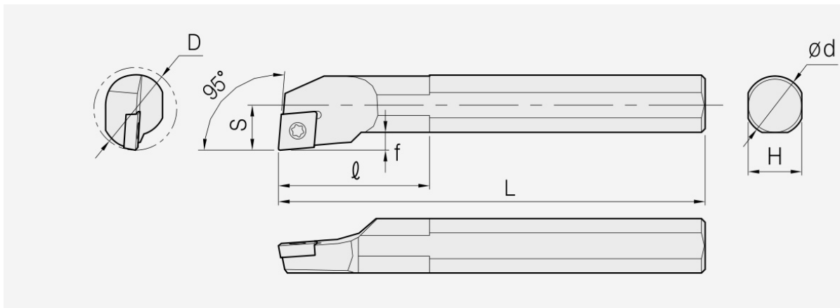
SCLP: holder dimension drawing; item dimensions and spare parts are listed in the corresponding tables.
