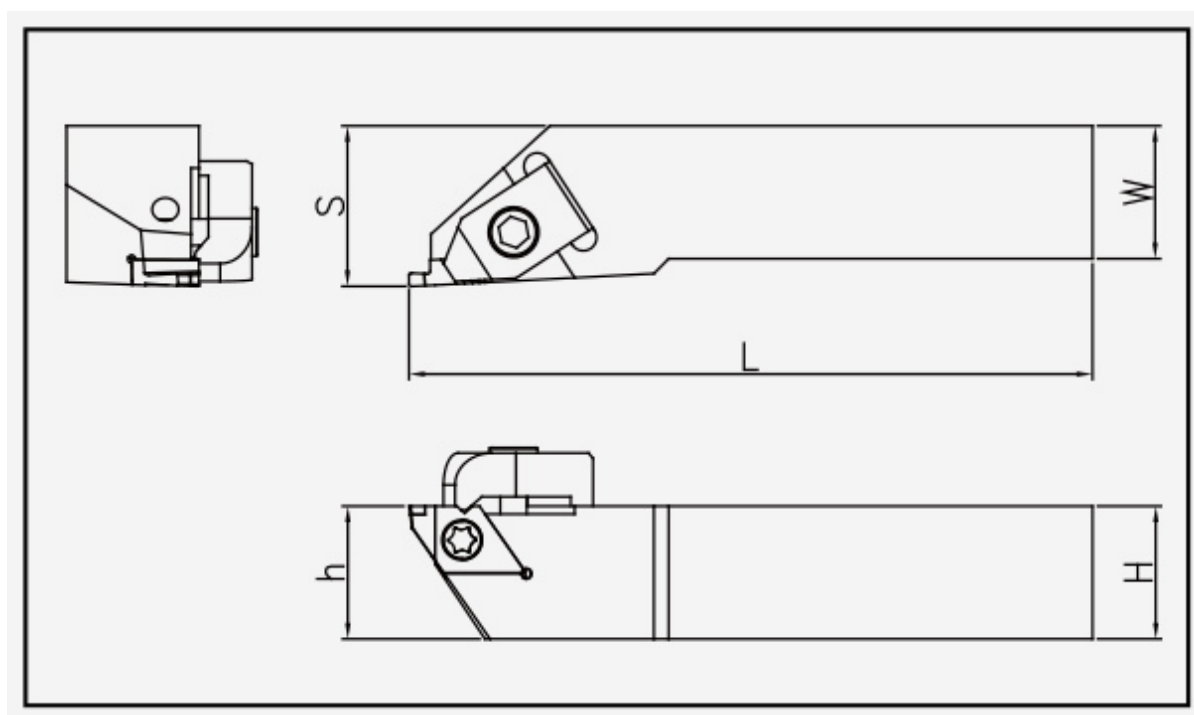
EDEH: holder dimension drawing; item dimensions and spare parts are listed in the corresponding tables.
