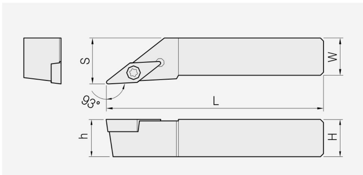
SVJB: holder dimension drawing; item dimensions and spare parts are listed in the corresponding tables.
