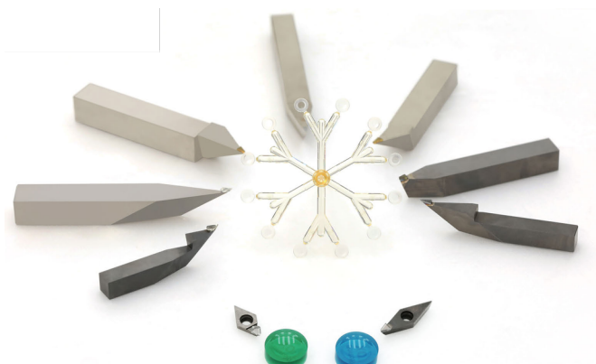
Single-crystal diamond cutting tools: Tool view.
