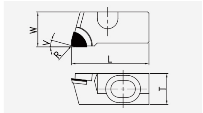
Insert: isolated dimensioned drawing with unchanged geometry symbols.
