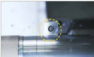
PCBN chipbreakers: SCM420 application examples: Component and machining view.
