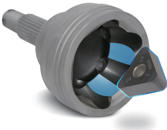
Outer-race hard turning.
