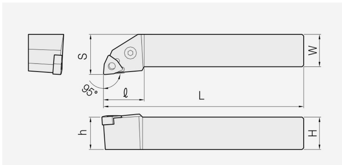
PNLN: holder dimension drawing; item dimensions and spare parts are listed in the corresponding tables.
