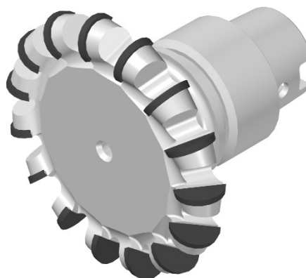
Design 66D-15Z-HSK32E(C).
