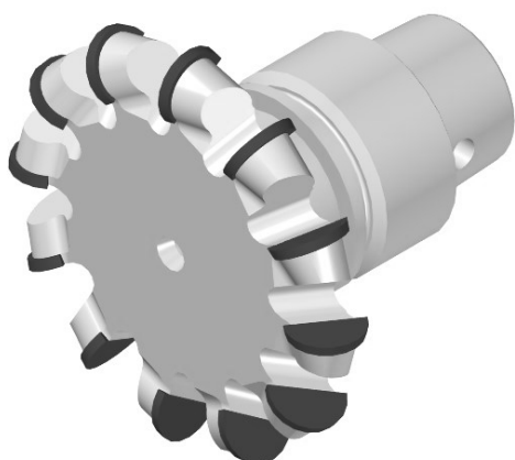
Design 66D-12Z-HSK32E(C).
