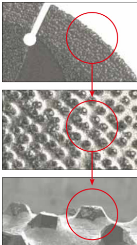
Diamond coating and detail views of SMART PADS: qualitative microscope images without a size scale.
