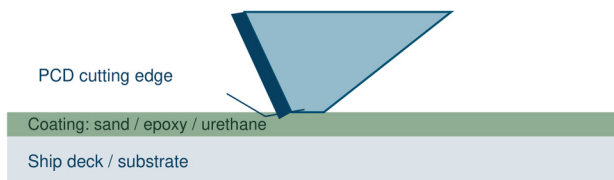
PCD coating removal principle: schematic, not to scale.
