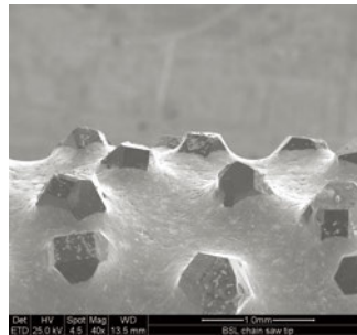
BSL chain-saw tip: micrograph with 1.0 mm scale
