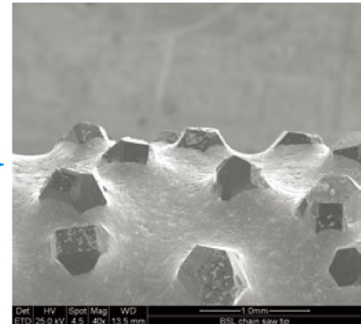
BSL chain-saw coating detail
